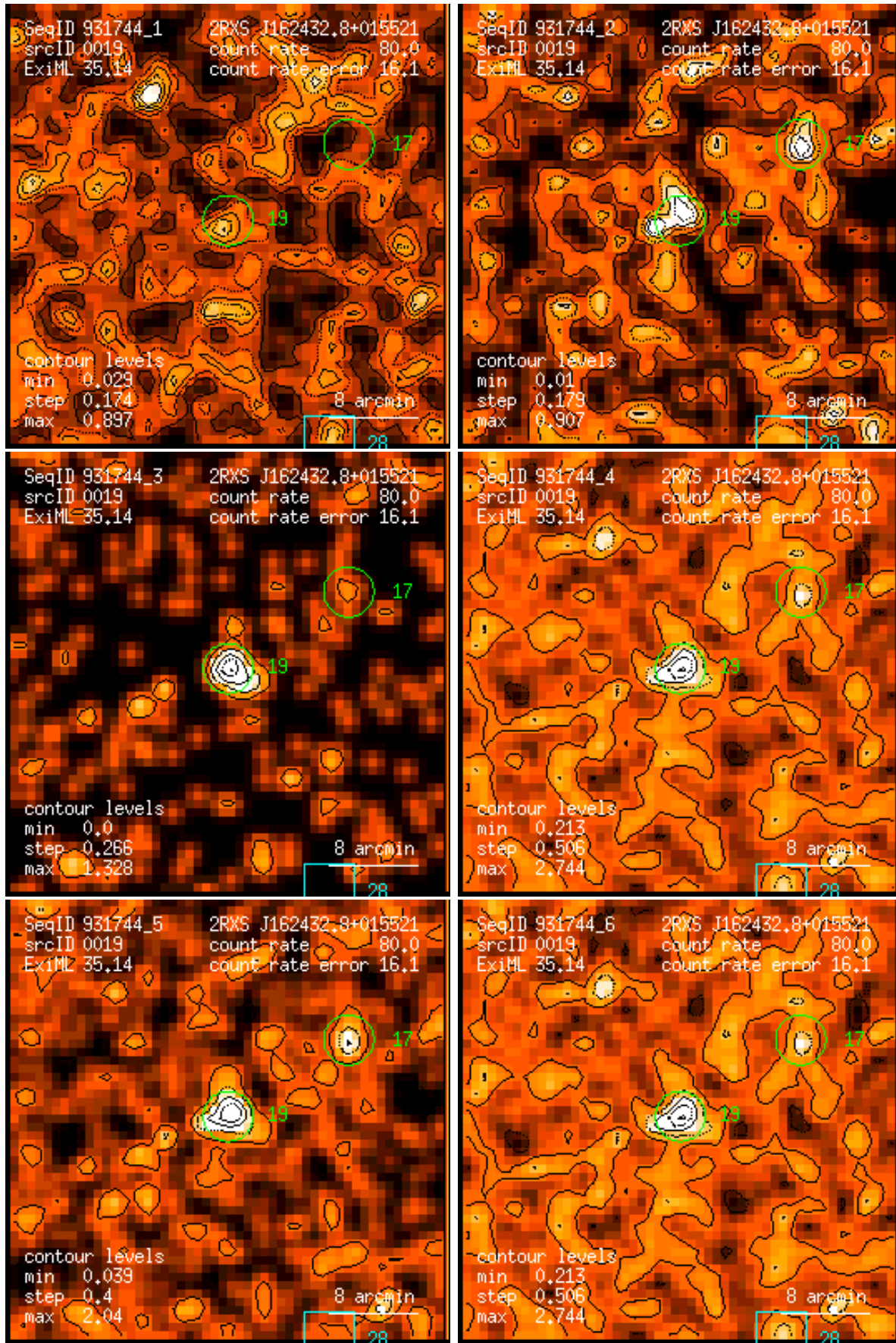
Figure 19: RASS 931744: detection 0019: band rate images, Gaussian filter: (1) PSPC channels 11 – 41, (2) 52 – 90, (3) 91 – 201, (4) 11 – 235, (5) 52 – 201, (6) 11 – 201. Broad band rates in counts/ks. Band rate contour levels in counts/ks/arcmin 2 .
