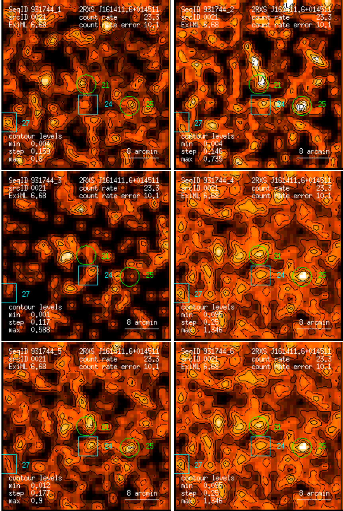
Figure 21: RASS 931744: detection 0021: band rate images, Gaussian filter: (1) PSPC channels 11 – 41, (2) 52 – 90, (3) 91 – 201, (4) 11 – 235, (5) 52 – 201, (6) 11 – 201. Broad band rates in counts/ks. Band rate contour levels in counts/ks/arcmin 2 .
