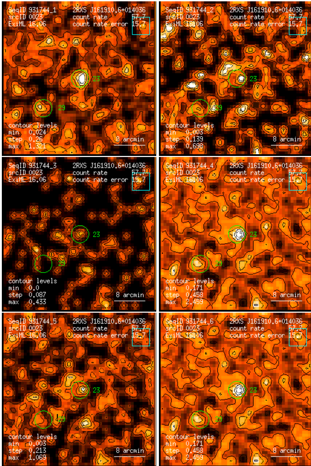
Figure 23: RASS 931744: detection 0023: band rate images, Gaussian filter: (1) PSPC channels 11 – 41, (2) 52 – 90, (3) 91 – 201, (4) 11 – 235, (5) 52 – 201, (6) 11 – 201. Broad band rates in counts/ks. Band rate contour levels in counts/ks/arcmin 2 .
