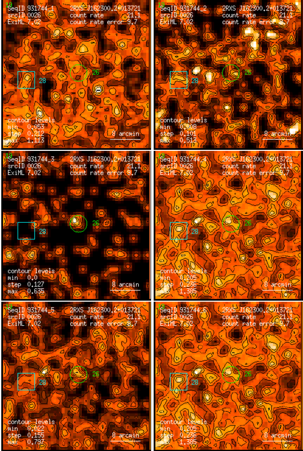
Figure 26: RASS 931744: detection 0026: band rate images, Gaussian filter: (1) PSPC channels 11 – 41, (2) 52 – 90, (3) 91 – 201, (4) 11 – 235, (5) 52 – 201, (6) 11 – 201. Broad band rates in counts/ks. Band rate contour levels in counts/ks/arcmin 2 .
