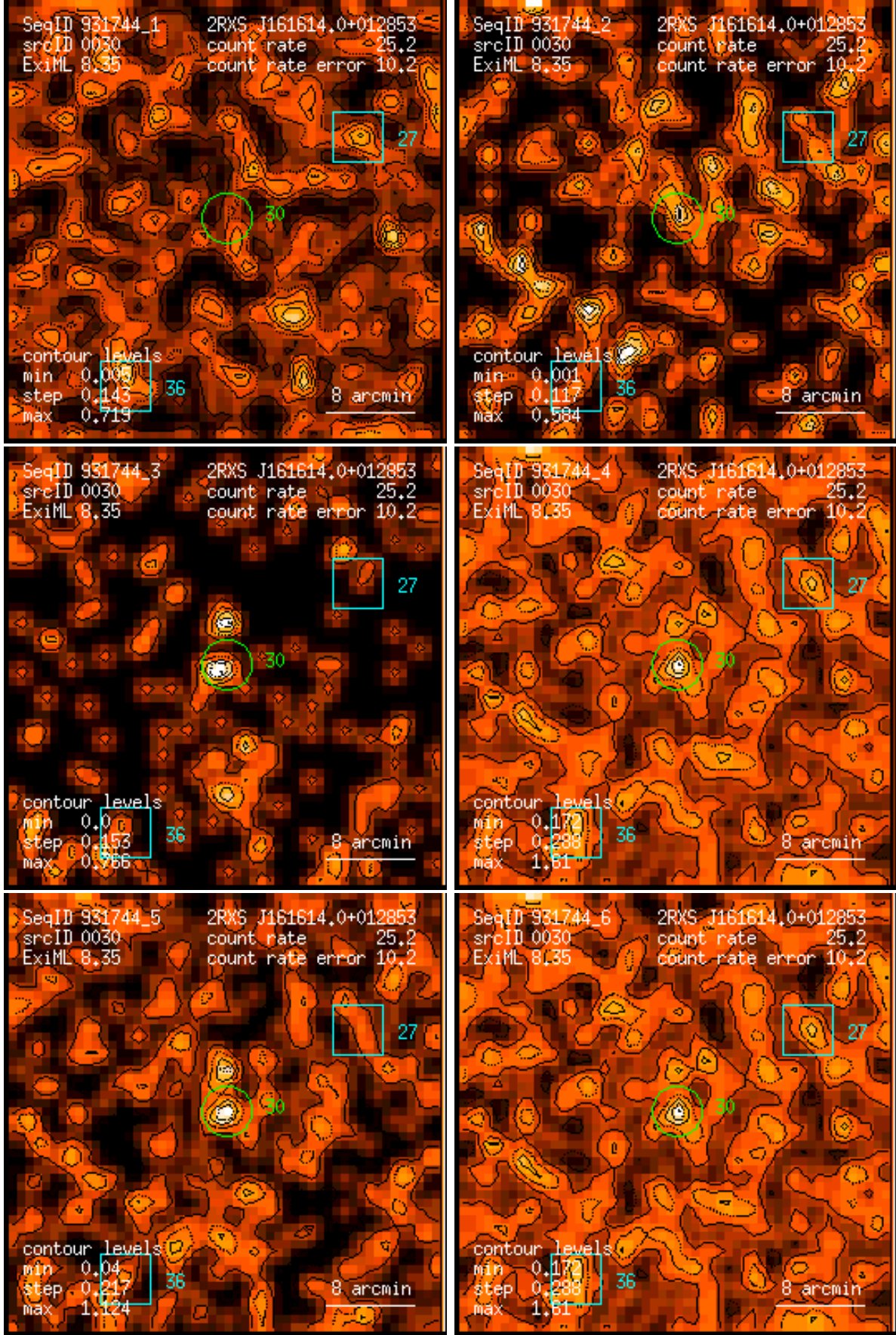
Figure 30: RASS 931744: detection 0030: band rate images, Gaussian filter: (1) PSPC channels 11 – 41, (2) 52 – 90, (3) 91 – 201, (4) 11 – 235, (5) 52 – 201, (6) 11 – 201. Broad band rates in counts/ks. Band rate contour levels in counts/ks/arcmin 2 .
