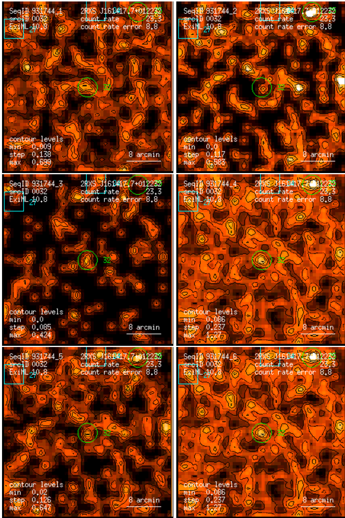
Figure 32: RASS 931744: detection 0032: band rate images, Gaussian filter: (1) PSPC channels 11 – 41, (2) 52 – 90, (3) 91 – 201, (4) 11 – 235, (5) 52 – 201, (6) 11 – 201. Broad band rates in counts/ks. Band rate contour levels in counts/ks/arcmin 2 .
