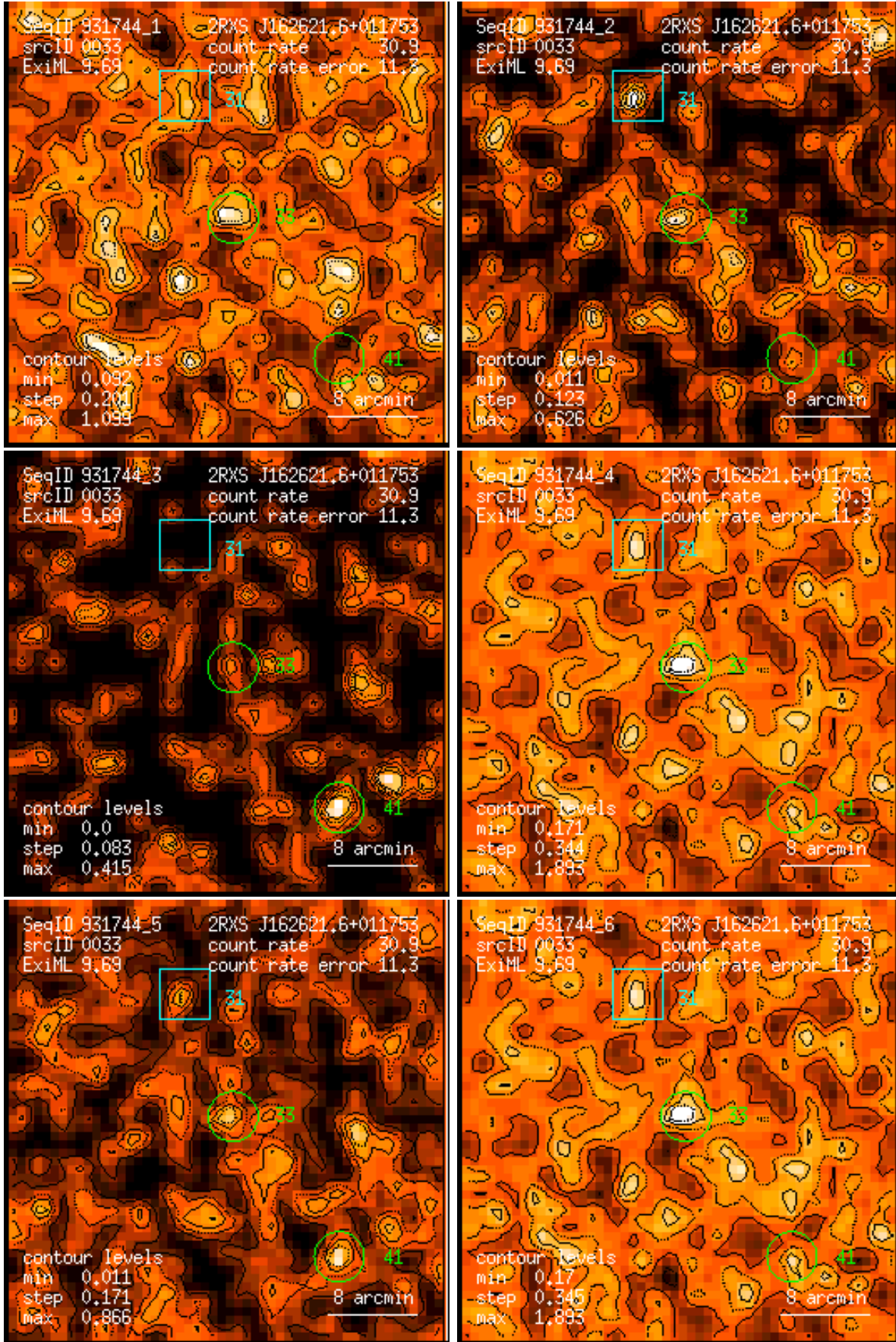
Figure 33: RASS 931744: detection 0033: band rate images, Gaussian filter: (1) PSPC channels 11 – 41, (2) 52 – 90, (3) 91 – 201, (4) 11 – 235, (5) 52 – 201, (6) 11 – 201. Broad band rates in counts/ks. Band rate contour levels in counts/ks/arcmin 2 .
