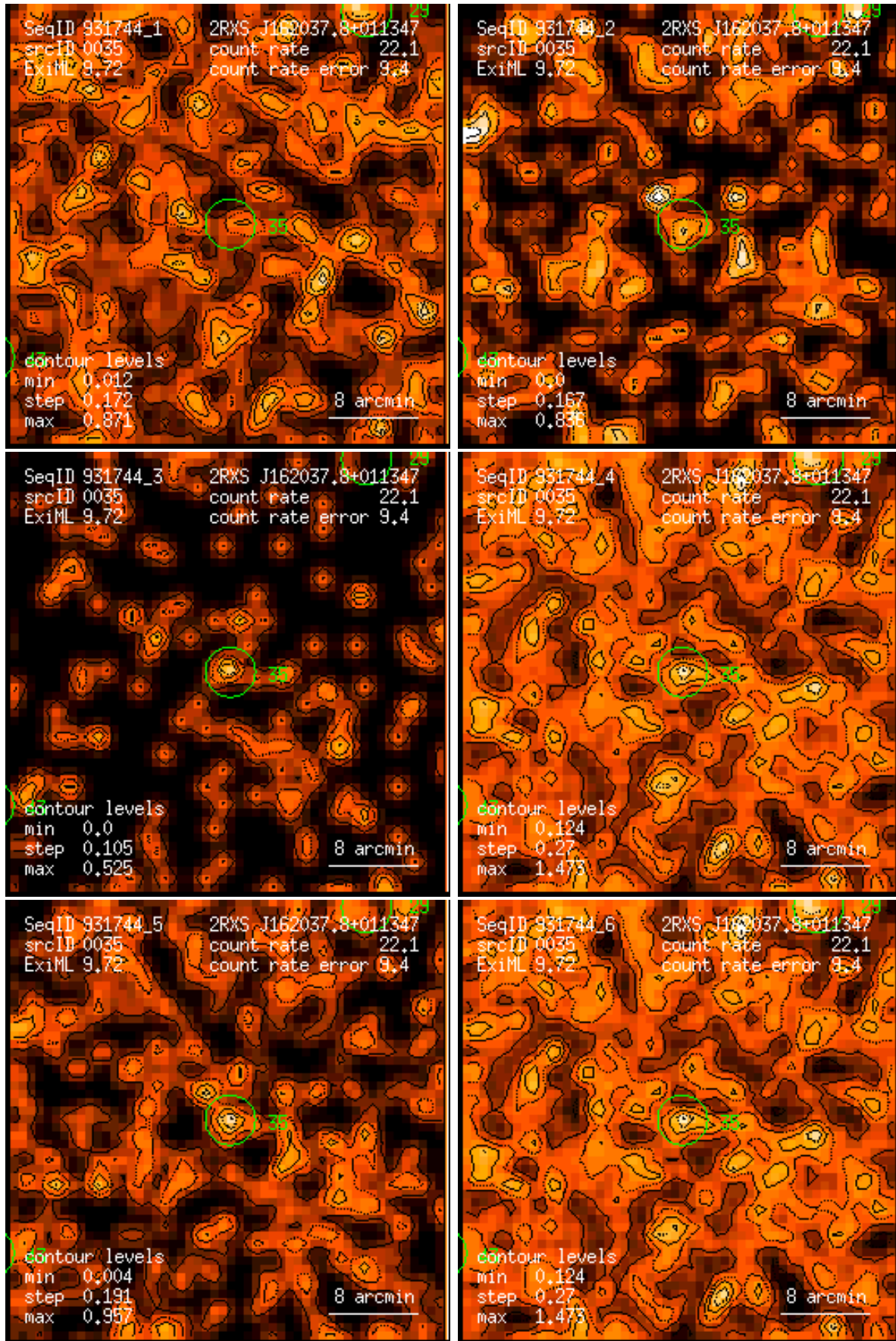
Figure 35: RASS 931744: detection 0035: band rate images, Gaussian filter: (1) PSPC channels 11 – 41, (2) 52 – 90, (3) 91 – 201, (4) 11 – 235, (5) 52 – 201, (6) 11 – 201. Broad band rates in counts/ks. Band rate contour levels in counts/ks/arcmin 2 .
