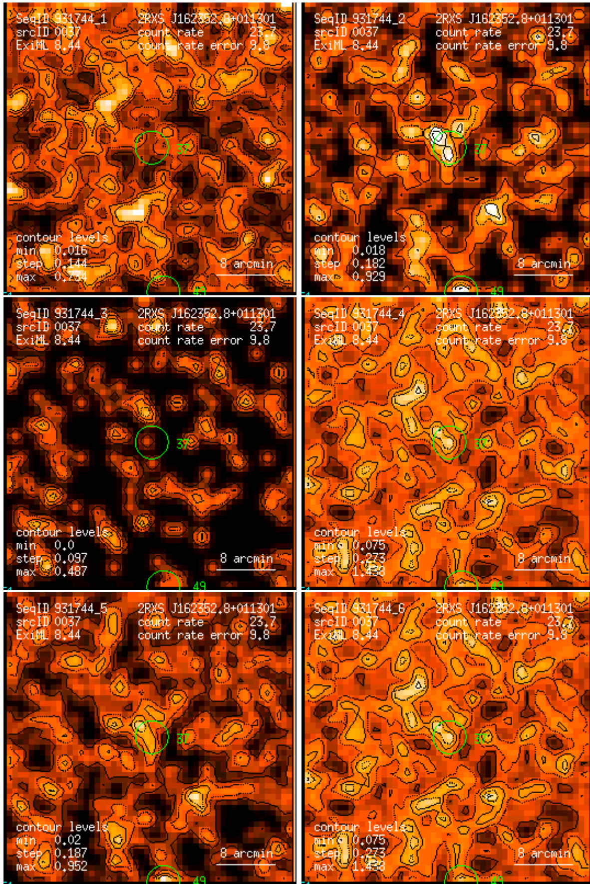
Figure 37: RASS 931744: detection 0037: band rate images, Gaussian filter: (1) PSPC channels 11 – 41, (2) 52 – 90, (3) 91 – 201, (4) 11 – 235, (5) 52 – 201, (6) 11 – 201. Broad band rates in counts/ks. Band rate contour levels in counts/ks/arcmin 2 .
