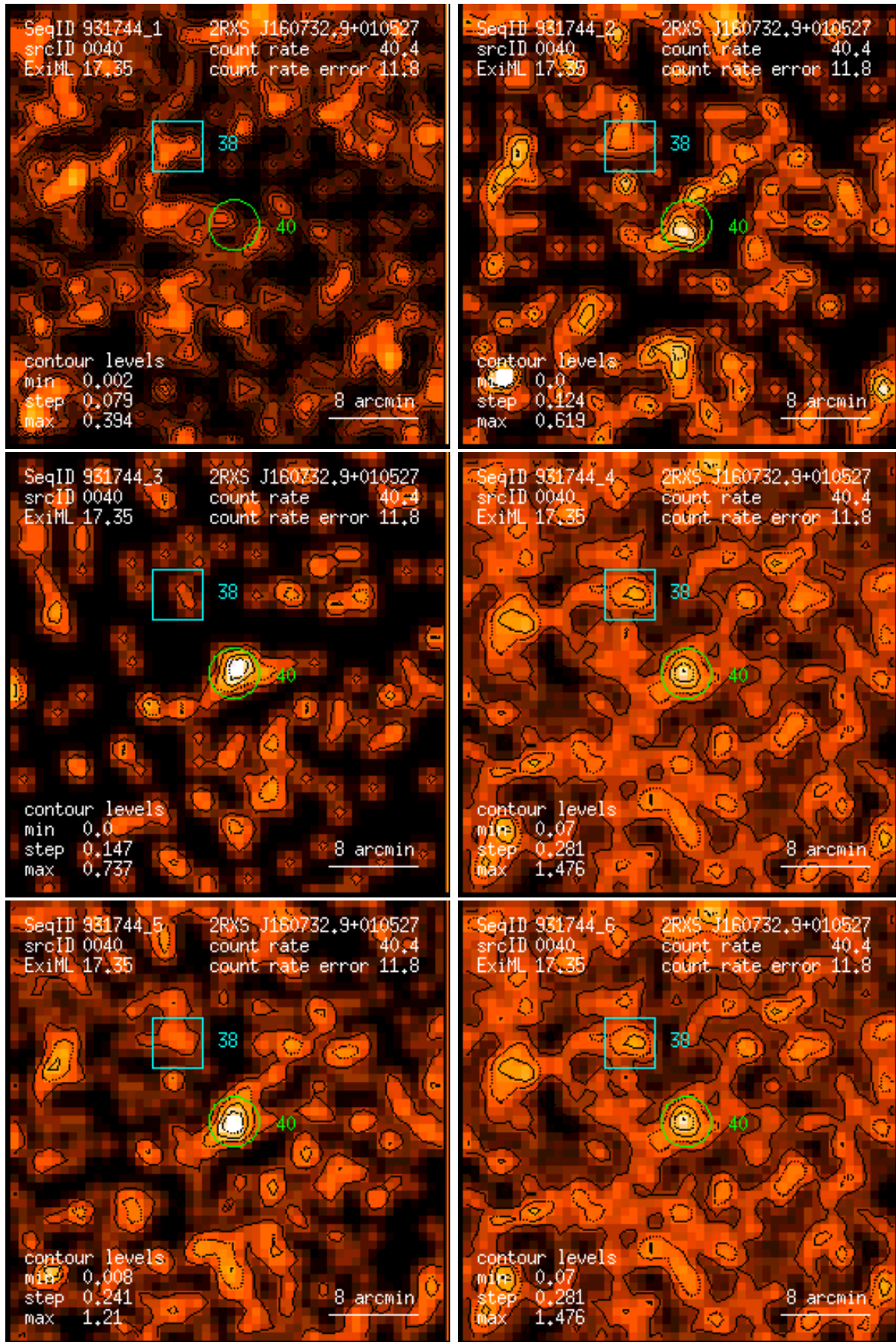
Figure 40: RASS 931744: detection 0040: band rate images, Gaussian filter: (1) PSPC channels 11 – 41, (2) 52 – 90, (3) 91 – 201, (4) 11 – 235, (5) 52 – 201, (6) 11 – 201. Broad band rates in counts/ks. Band rate contour levels in counts/ks/arcmin 2 .
