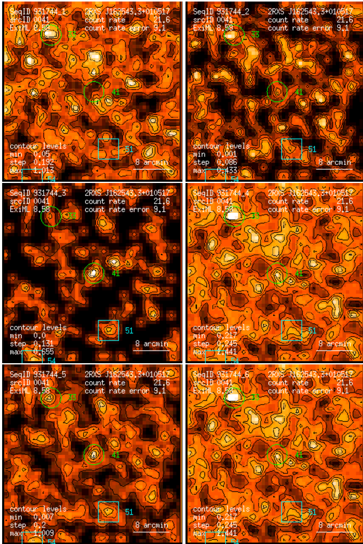
Figure 41: RASS 931744: detection 0041: band rate images, Gaussian filter: (1) PSPC channels 11 – 41, (2) 52 – 90, (3) 91 – 201, (4) 11 – 235, (5) 52 – 201, (6) 11 – 201. Broad band rates in counts/ks. Band rate contour levels in counts/ks/arcmin 2 .
