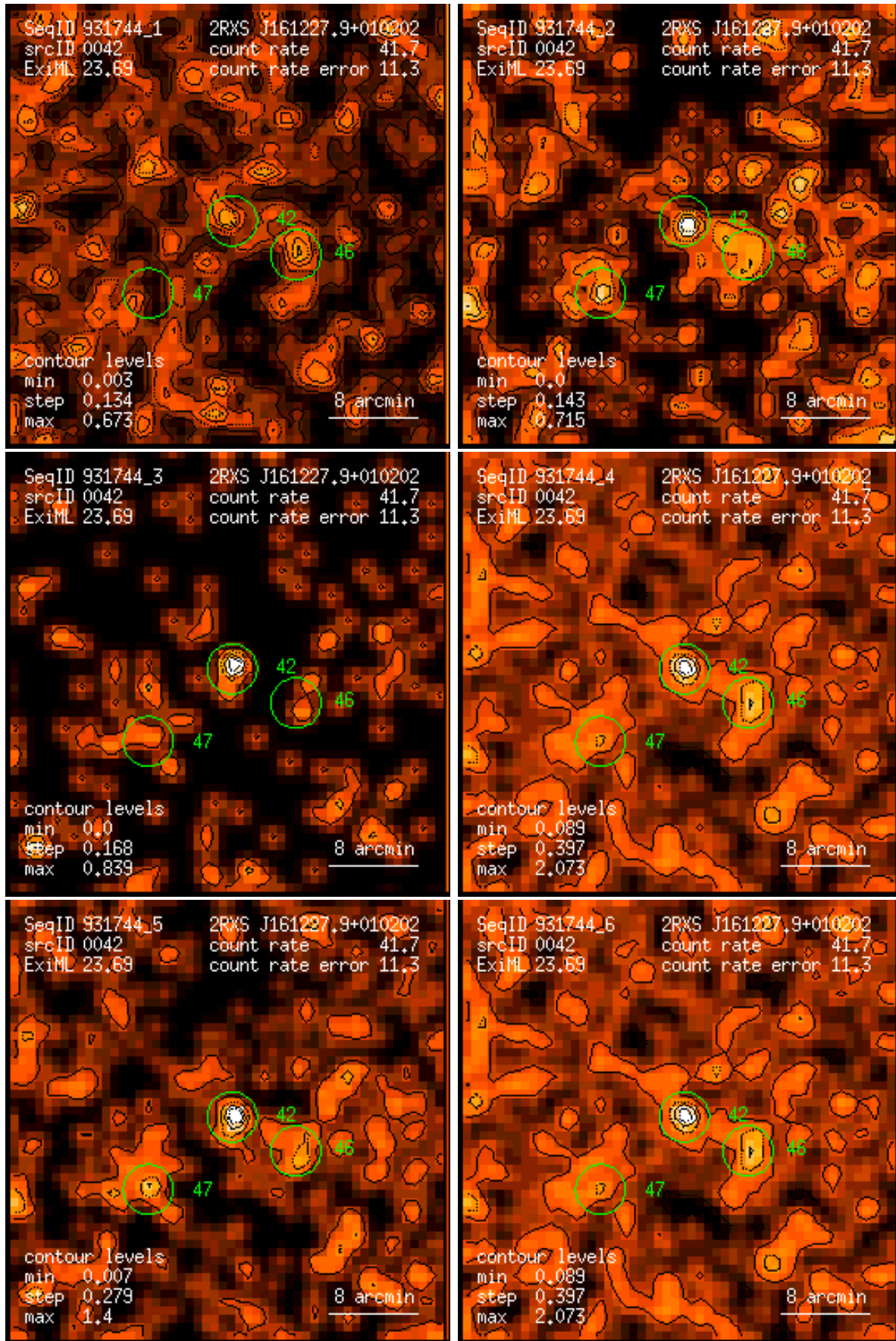
Figure 42: RASS 931744: detection 0042: band rate images, Gaussian filter: (1) PSPC channels 11 – 41, (2) 52 – 90, (3) 91 – 201, (4) 11 – 235, (5) 52 – 201, (6) 11 – 201. Broad band rates in counts/ks. Band rate contour levels in counts/ks/arcmin 2 .
