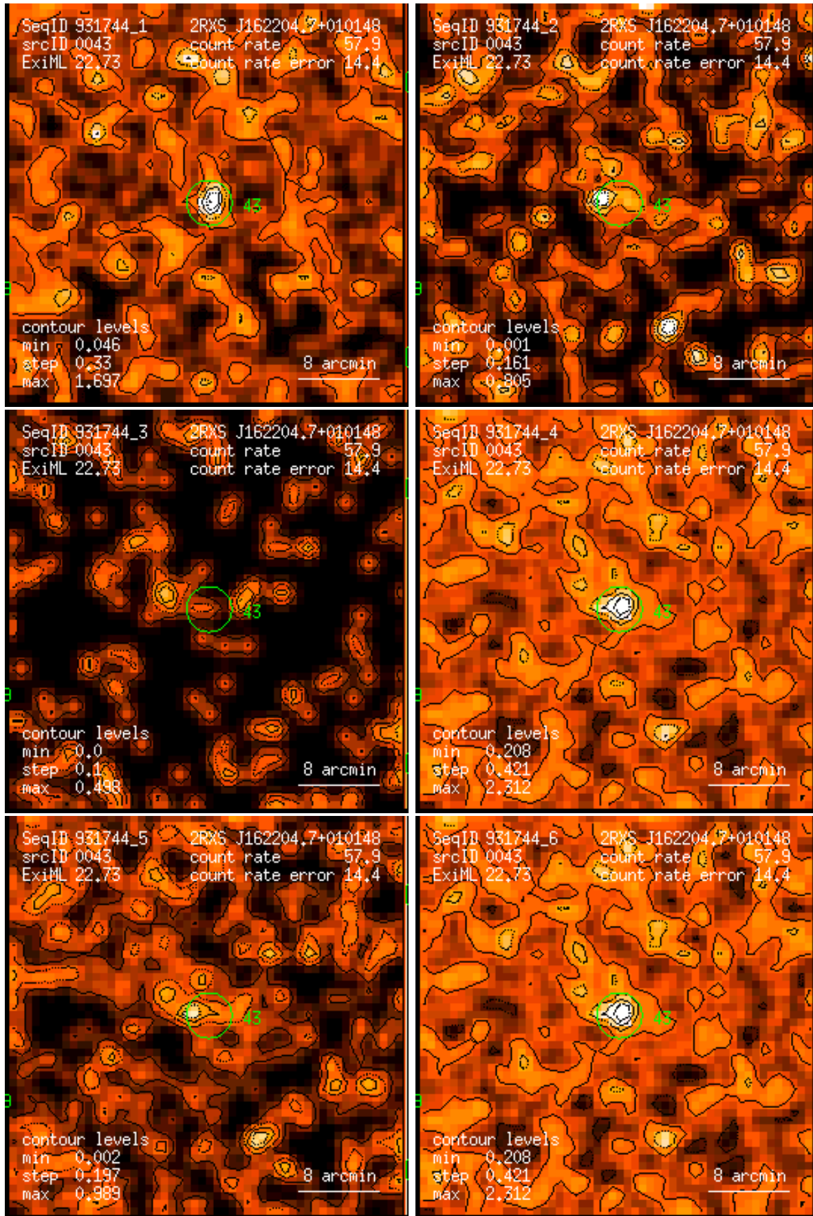
Figure 43: RASS 931744: detection 0043: band rate images, Gaussian filter: (1) PSPC channels 11 – 41, (2) 52 – 90, (3) 91 – 201, (4) 11 – 235, (5) 52 – 201, (6) 11 – 201. Broad band rates in counts/ks. Band rate contour levels in counts/ks/arcmin 2 .
