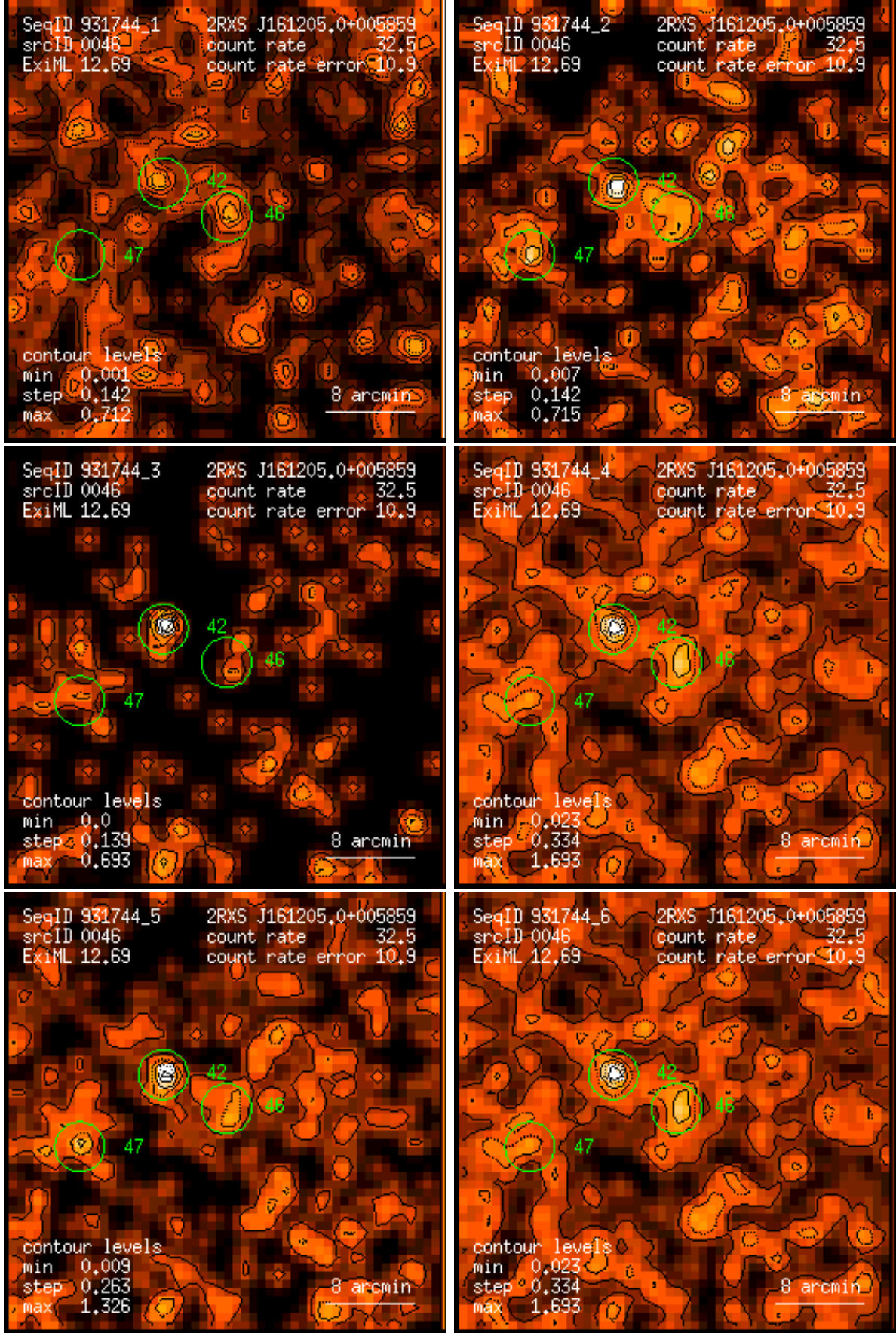
Figure 46: RASS 931744: detection 0046: band rate images, Gaussian filter: (1) PSPC channels 11 – 41, (2) 52 – 90, (3) 91 – 201, (4) 11 – 235, (5) 52 – 201, (6) 11 – 201. Broad band rates in counts/ks. Band rate contour levels in counts/ks/arcmin 2 .
