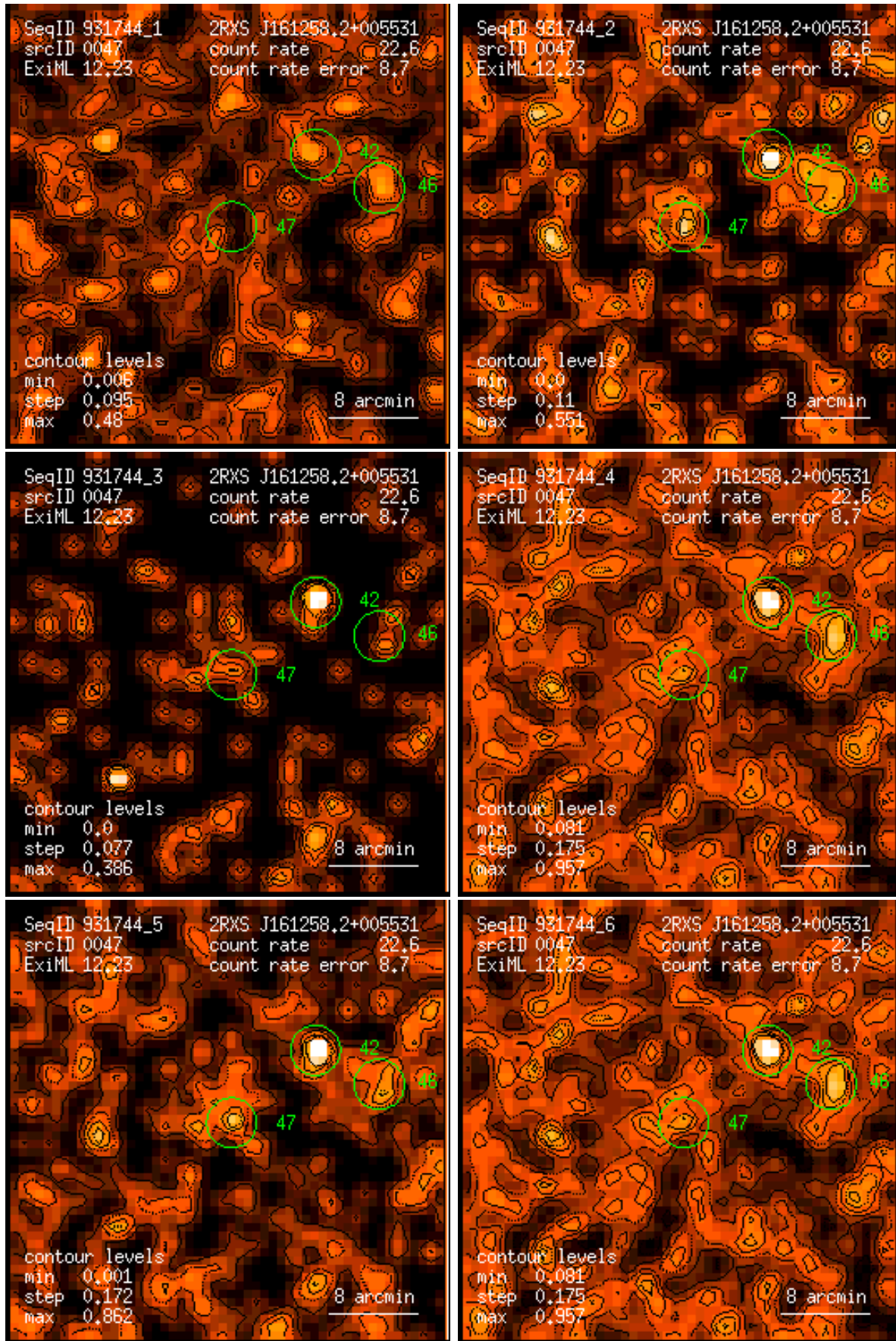
Figure 47: RASS 931744: detection 0047: band rate images, Gaussian filter: (1) PSPC channels 11 – 41, (2) 52 – 90, (3) 91 – 201, (4) 11 – 235, (5) 52 – 201, (6) 11 – 201. Broad band rates in counts/ks. Band rate contour levels in counts/ks/arcmin 2 .
