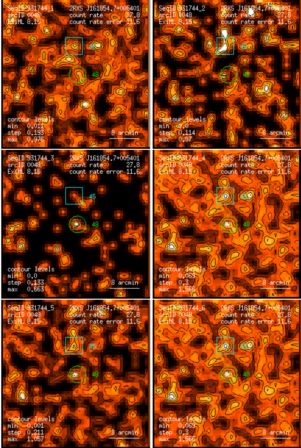
Figure 48: RASS 931744: detection 0048: band rate images, Gaussian filter: (1) PSPC channels 11 – 41, (2) 52 – 90, (3) 91 – 201, (4) 11 – 235, (5) 52 – 201, (6) 11 – 201. Broad band rates in counts/ks. Band rate contour levels in counts/ks/arcmin 2 .
