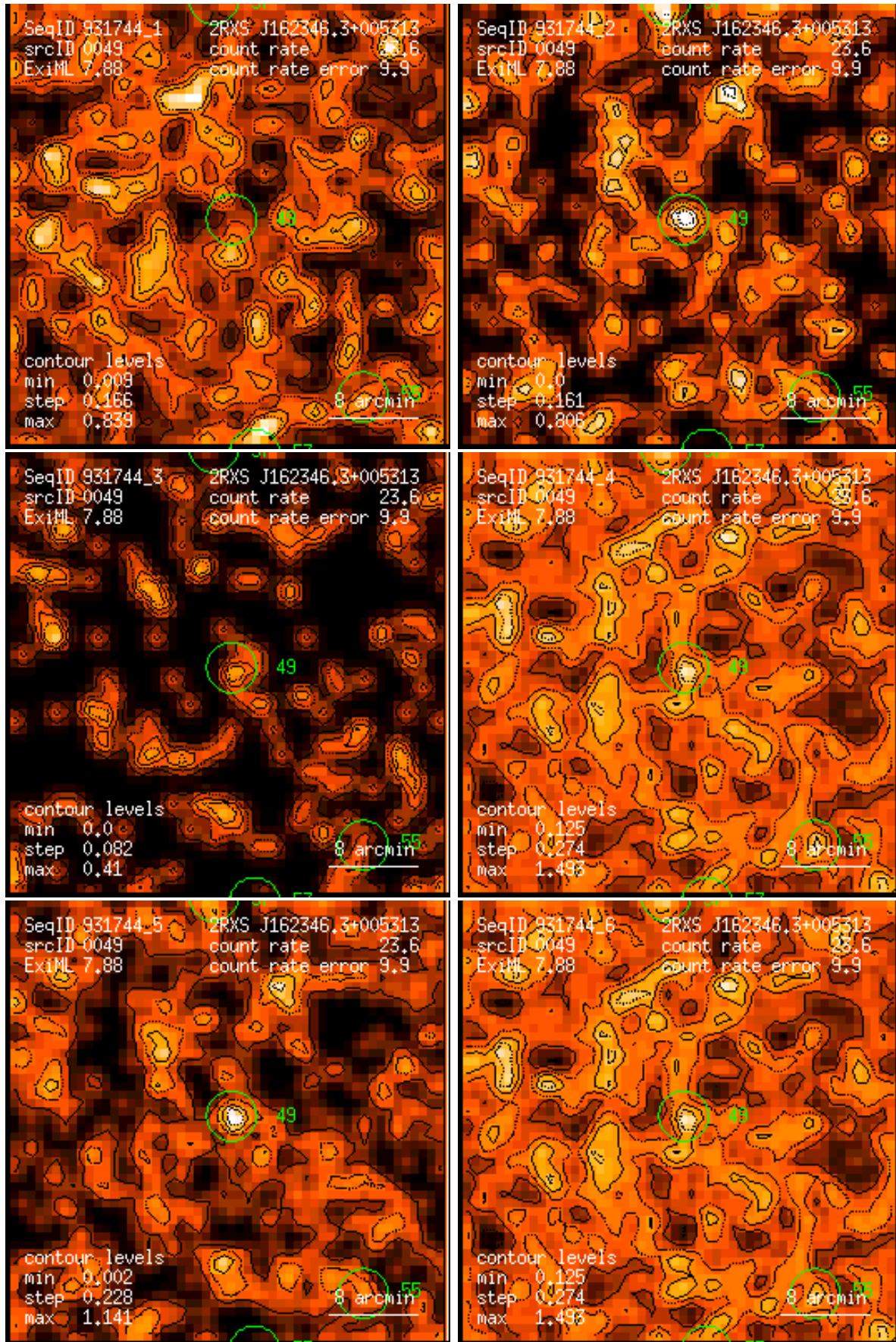
Figure 49: RASS 931744: detection 0049: band rate images, Gaussian filter: (1) PSPC channels 11 – 41, (2) 52 – 90, (3) 91 – 201, (4) 11 – 235, (5) 52 – 201, (6) 11 – 201. Broad band rates in counts/ks. Band rate contour levels in counts/ks/arcmin 2 .
