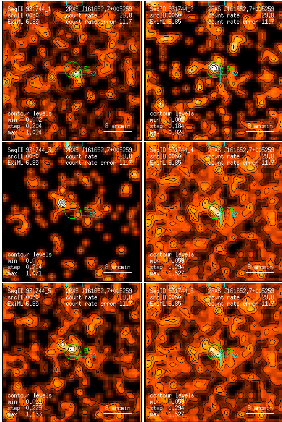
Figure 50: RASS 931744: detection 0050: band rate images, Gaussian filter: (1) PSPC channels 11 – 41, (2) 52 – 90, (3) 91 – 201, (4) 11 – 235, (5) 52 – 201, (6) 11 – 201. Broad band rates in counts/ks. Band rate contour levels in counts/ks/arcmin 2 .
