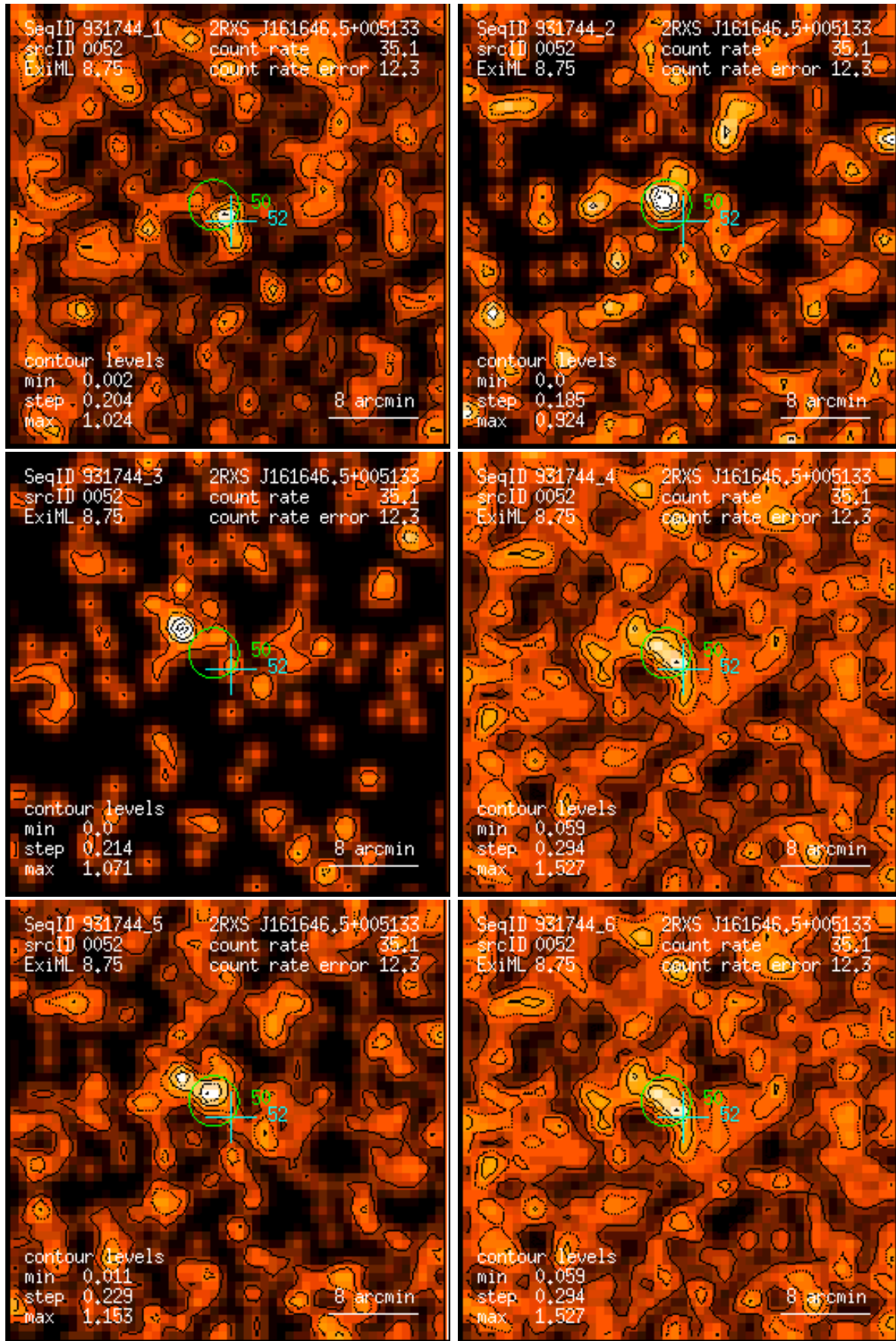
Figure 52: RASS 931744: detection 0052: band rate images, Gaussian filter: (1) PSPC channels 11 – 41, (2) 52 – 90, (3) 91 – 201, (4) 11 – 235, (5) 52 – 201, (6) 11 – 201. Broad band rates in counts/ks. Band rate contour levels in counts/ks/arcmin 2 .
