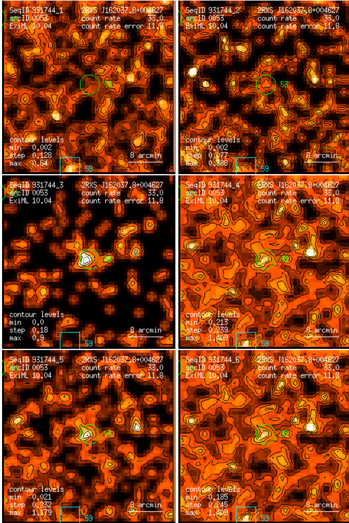
Figure 53: RASS 931744: detection 0053: band rate images, Gaussian filter: (1) PSPC channels 11 – 41, (2) 52 – 90, (3) 91 – 201, (4) 11 – 235, (5) 52 – 201, (6) 11 – 201. Broad band rates in counts/ks. Band rate contour levels in counts/ks/arcmin 2 .
