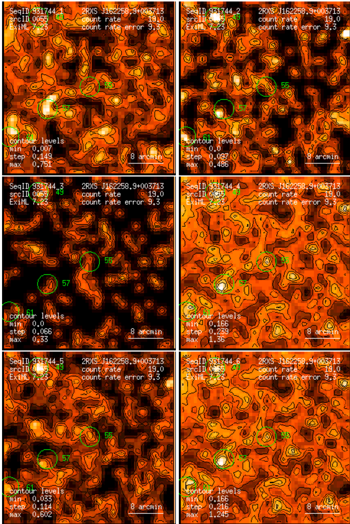
Figure 55: RASS 931744: detection 0055: band rate images, Gaussian filter: (1) PSPC channels 11 – 41, (2) 52 – 90, (3) 91 – 201, (4) 11 – 235, (5) 52 – 201, (6) 11 – 201. Broad band rates in counts/ks. Band rate contour levels in counts/ks/arcmin 2 .
