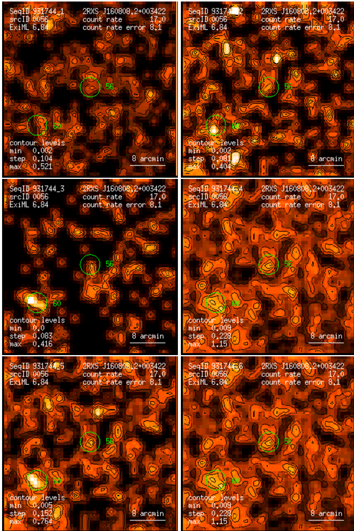
Figure 56: RASS 931744: detection 0056: band rate images, Gaussian filter: (1) PSPC channels 11 – 41, (2) 52 – 90, (3) 91 – 201, (4) 11 – 235, (5) 52 – 201, (6) 11 – 201. Broad band rates in counts/ks. Band rate contour levels in counts/ks/arcmin 2 .
