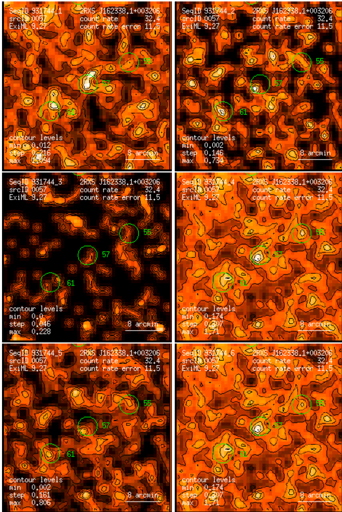
Figure 57: RASS 931744: detection 0057: band rate images, Gaussian filter: (1) PSPC channels 11 – 41, (2) 52 – 90, (3) 91 – 201, (4) 11 – 235, (5) 52 – 201, (6) 11 – 201. Broad band rates in counts/ks. Band rate contour levels in counts/ks/arcmin 2 .
