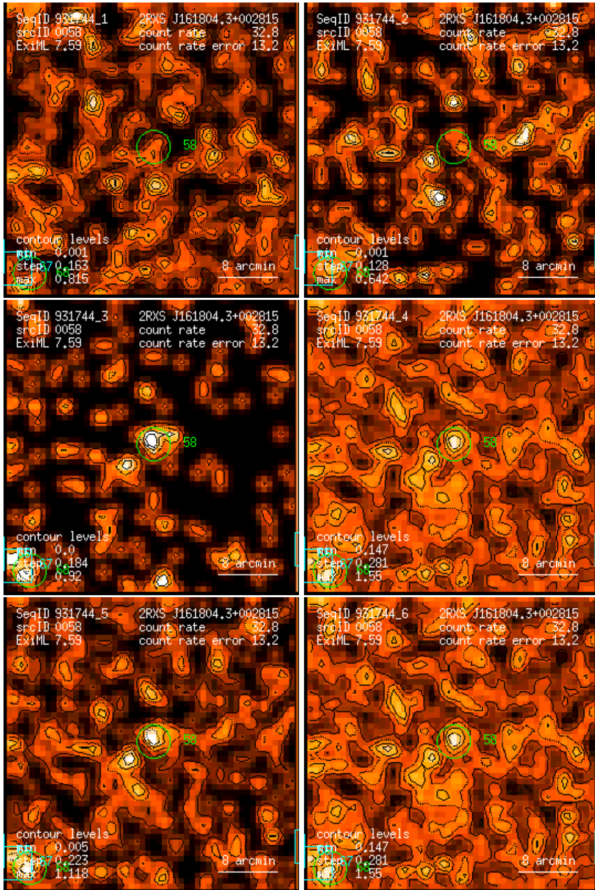
Figure 58: RASS 931744: detection 0058: band rate images, Gaussian filter: (1) PSPC channels 11 – 41, (2) 52 – 90, (3) 91 – 201, (4) 11 – 235, (5) 52 – 201, (6) 11 – 201. Broad band rates in counts/ks. Band rate contour levels in counts/ks/arcmin 2 .
