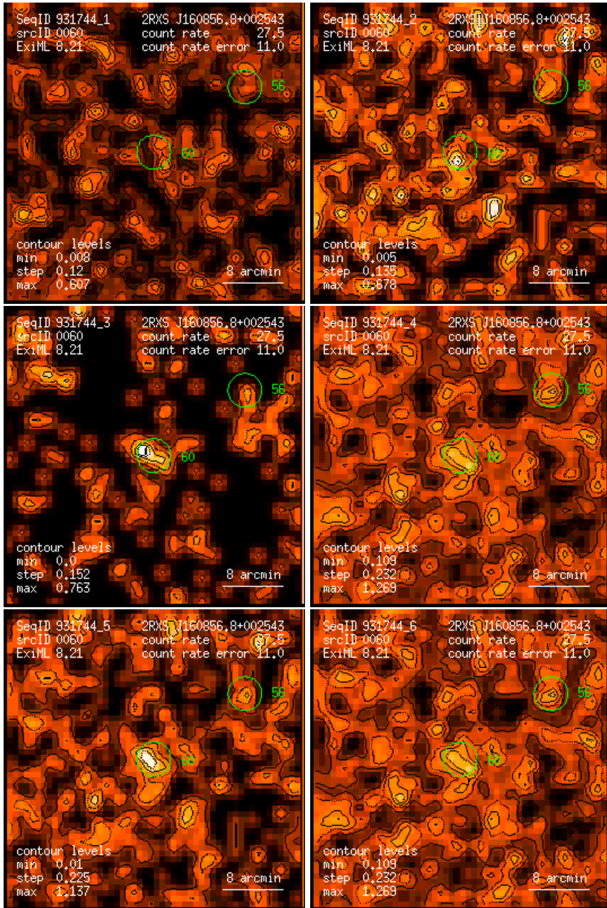
Figure 60: RASS 931744: detection 0060: band rate images, Gaussian filter: (1) PSPC channels 11 – 41, (2) 52 – 90, (3) 91 – 201, (4) 11 – 235, (5) 52 – 201, (6) 11 – 201. Broad band rates in counts/ks. Band rate contour levels in counts/ks/arcmin 2 .
