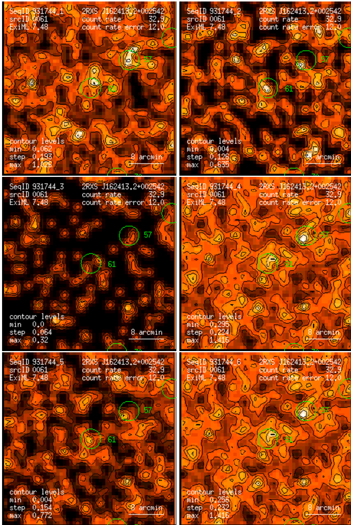
Figure 61: RASS 931744: detection 0061: band rate images, Gaussian filter: (1) PSPC channels 11 – 41, (2) 52 – 90, (3) 91 – 201, (4) 11 – 235, (5) 52 – 201, (6) 11 – 201. Broad band rates in counts/ks. Band rate contour levels in counts/ks/arcmin 2 .
