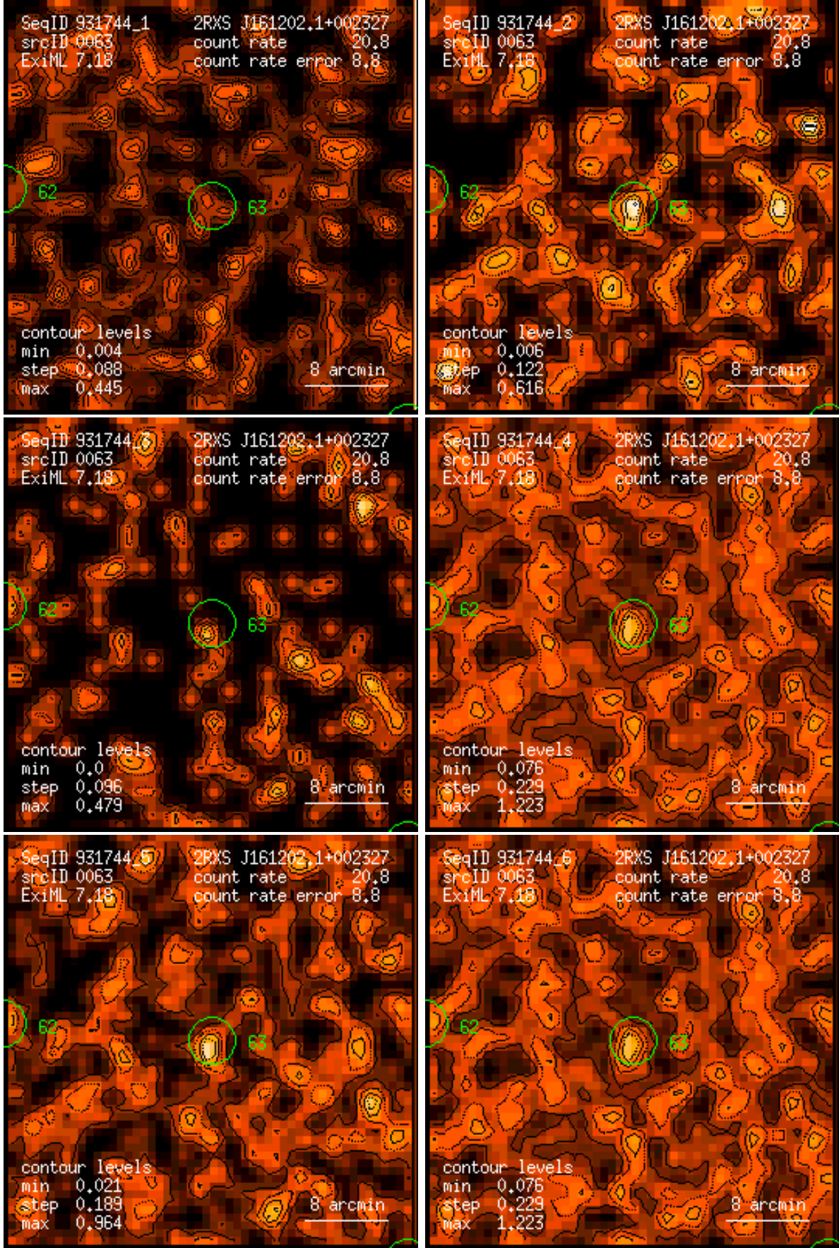
Figure 63: RASS 931744: detection 0063: band rate images, Gaussian filter: (1) PSPC channels 11 – 41, (2) 52 – 90, (3) 91 – 201, (4) 11 – 235, (5) 52 – 201, (6) 11 – 201. Broad band rates in counts/ks. Band rate contour levels in counts/ks/arcmin 2 .
