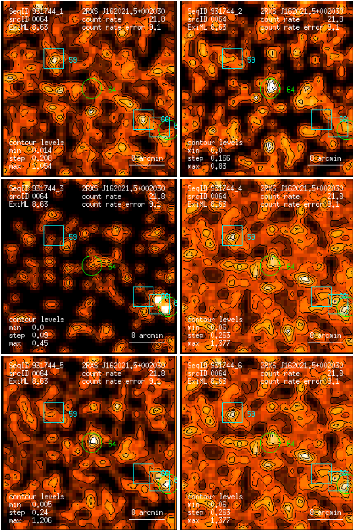
Figure 64: RASS 931744: detection 0064: band rate images, Gaussian filter: (1) PSPC channels 11 – 41, (2) 52 – 90, (3) 91 – 201, (4) 11 – 235, (5) 52 – 201, (6) 11 – 201. Broad band rates in counts/ks. Band rate contour levels in counts/ks/arcmin 2 .
