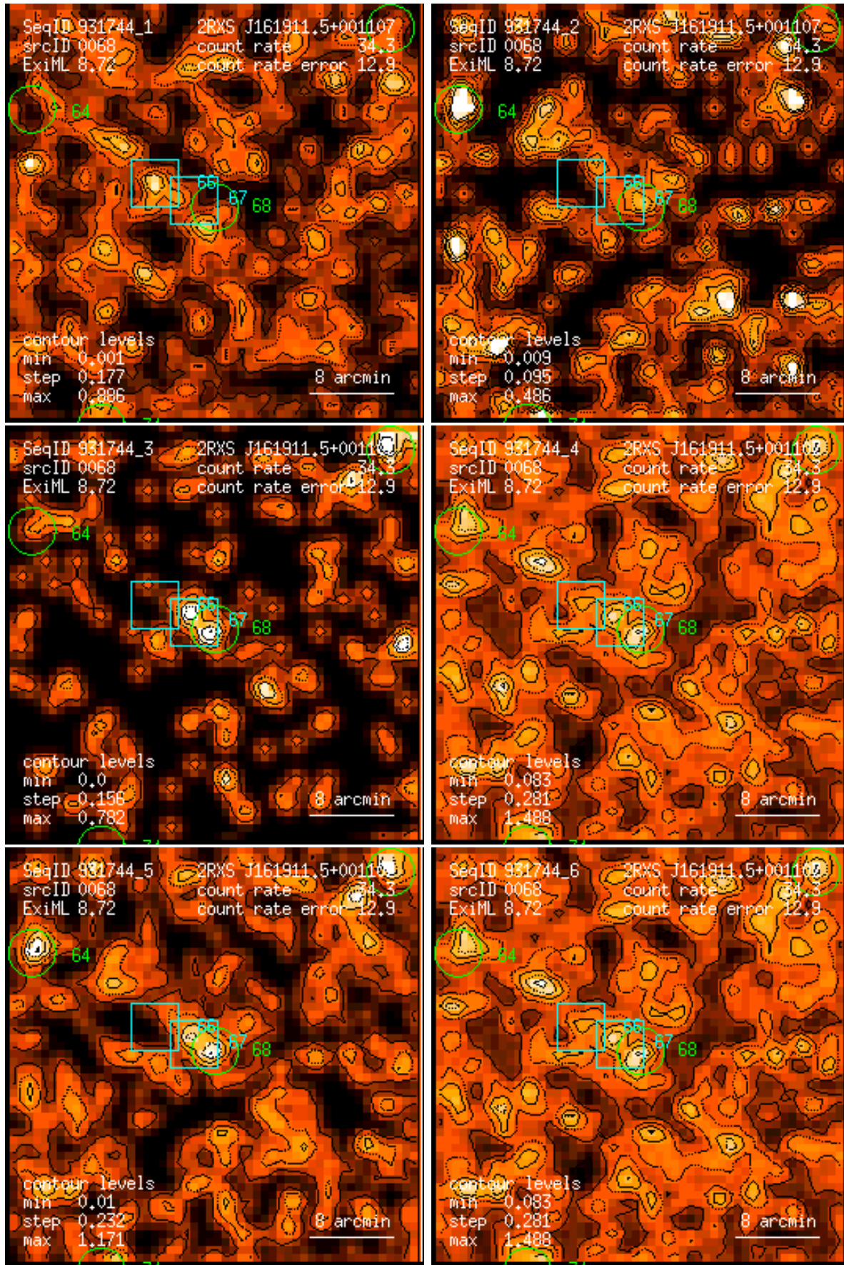
Figure 68: RASS 931744: detection 0068: band rate images, Gaussian filter: (1) PSPC channels 11 – 41, (2) 52 – 90, (3) 91 – 201, (4) 11 – 235, (5) 52 – 201, (6) 11 – 201. Broad band rates in counts/ks. Band rate contour levels in counts/ks/arcmin 2 .
