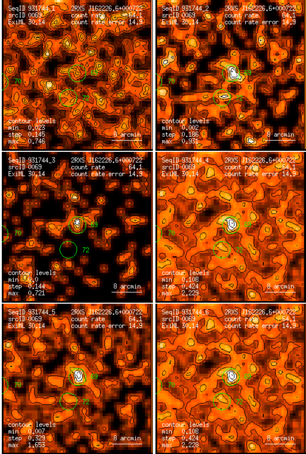
Figure 69: RASS 931744: detection 0069: band rate images, Gaussian filter: (1) PSPC channels 11 – 41, (2) 52 – 90, (3) 91 – 201, (4) 11 – 235, (5) 52 – 201, (6) 11 – 201. Broad band rates in counts/ks. Band rate contour levels in counts/ks/arcmin 2 .
