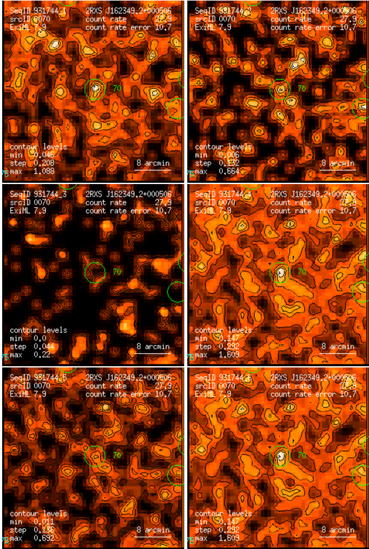
Figure 70: RASS 931744: detection 0070: band rate images, Gaussian filter: (1) PSPC channels 11 – 41, (2) 52 – 90, (3) 91 – 201, (4) 11 – 235, (5) 52 – 201, (6) 11 – 201. Broad band rates in counts/ks. Band rate contour levels in counts/ks/arcmin 2 .
