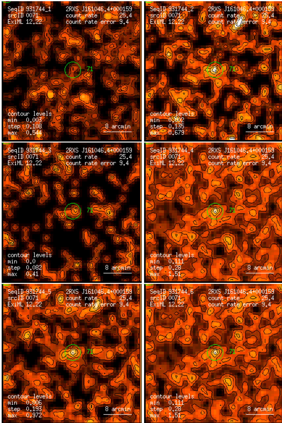
Figure 71: RASS 931744: detection 0071: band rate images, Gaussian filter: (1) PSPC channels 11 – 41, (2) 52 – 90, (3) 91 – 201, (4) 11 – 235, (5) 52 – 201, (6) 11 – 201. Broad band rates in counts/ks. Band rate contour levels in counts/ks/arcmin 2 .
