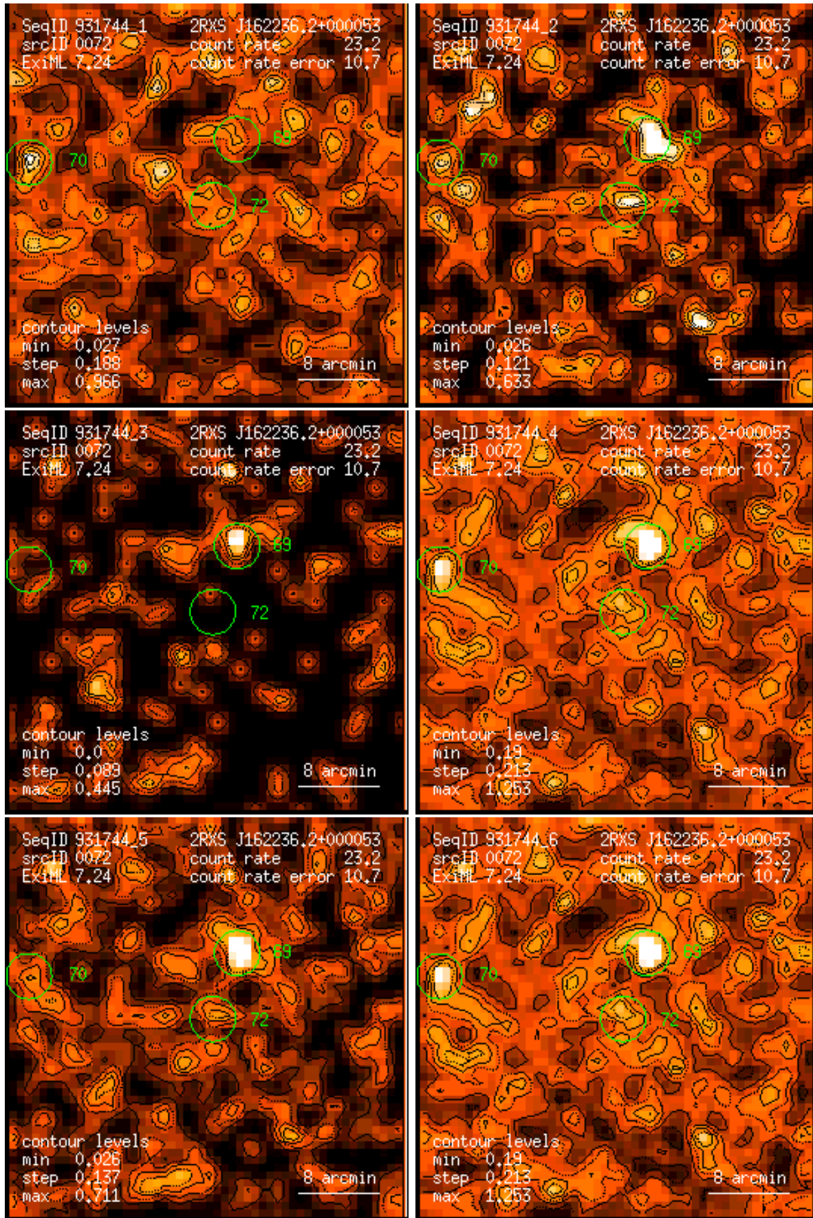
Figure 72: RASS 931744: detection 0072: band rate images, Gaussian filter: (1) PSPC channels 11 – 41, (2) 52 – 90, (3) 91 – 201, (4) 11 – 235, (5) 52 – 201, (6) 11 – 201. Broad band rates in counts/ks. Band rate contour levels in counts/ks/arcmin 2 .
