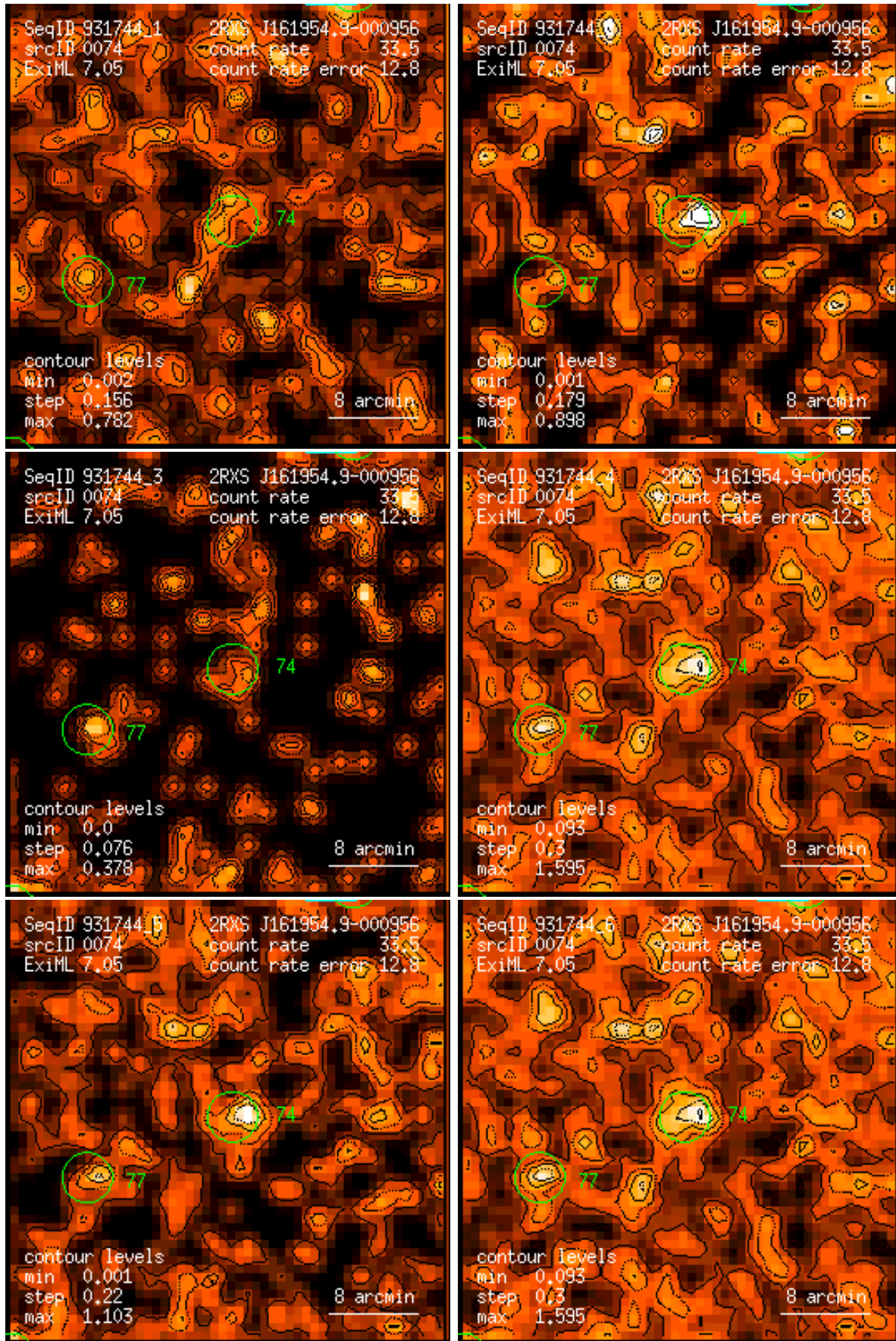
Figure 74: RASS 931744: detection 0074: band rate images, Gaussian filter: (1) PSPC channels 11 – 41, (2) 52 – 90, (3) 91 – 201, (4) 11 – 235, (5) 52 – 201, (6) 11 – 201. Broad band rates in counts/ks. Band rate contour levels in counts/ks/arcmin 2 .
