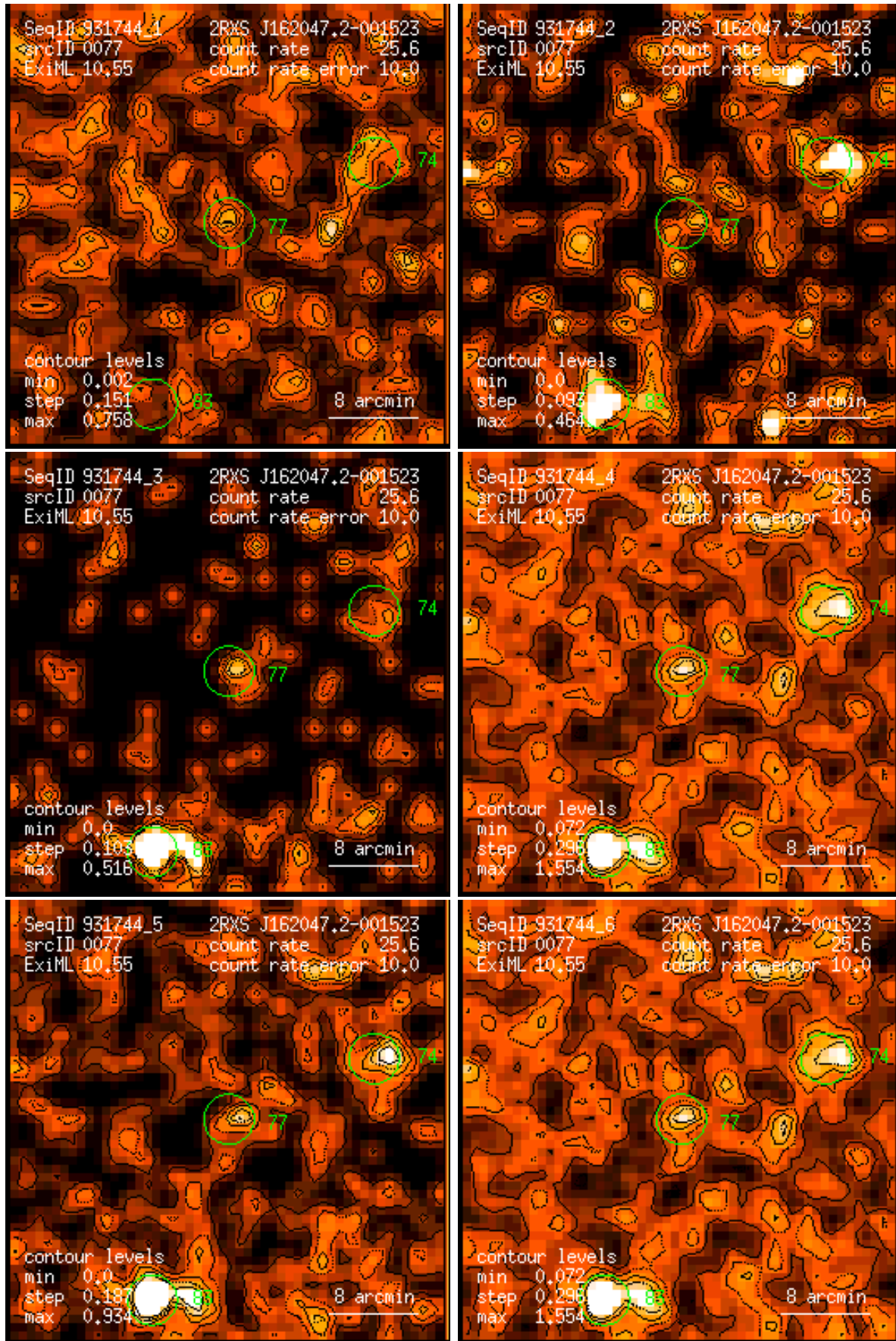
Figure 77: RASS 931744: detection 0077: band rate images, Gaussian filter: (1) PSPC channels 11 – 41, (2) 52 – 90, (3) 91 – 201, (4) 11 – 235, (5) 52 – 201, (6) 11 – 201. Broad band rates in counts/ks. Band rate contour levels in counts/ks/arcmin 2 .
