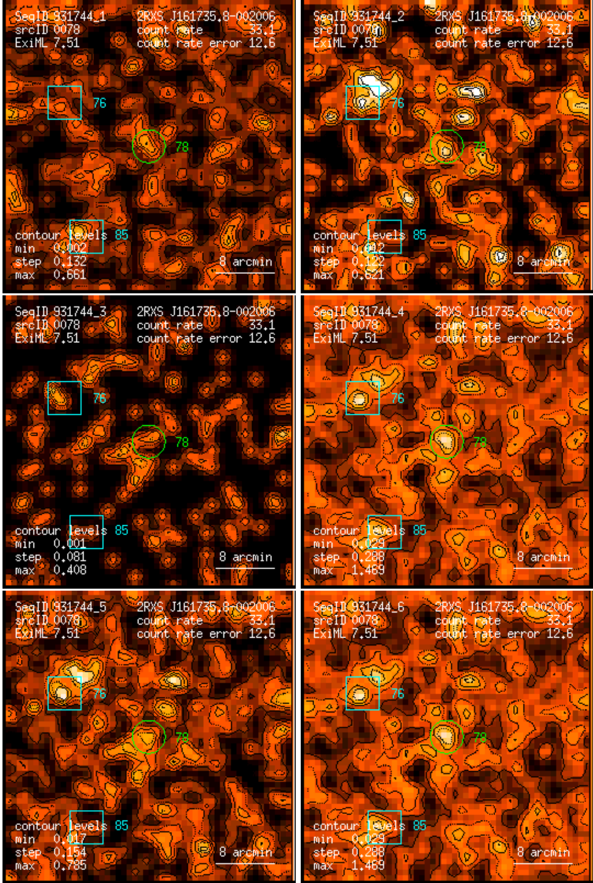
Figure 78: RASS 931744: detection 0078: band rate images, Gaussian filter: (1) PSPC channels 11 – 41, (2) 52 – 90, (3) 91 – 201, (4) 11 – 235, (5) 52 – 201, (6) 11 – 201. Broad band rates in counts/ks. Band rate contour levels in counts/ks/arcmin 2 .
