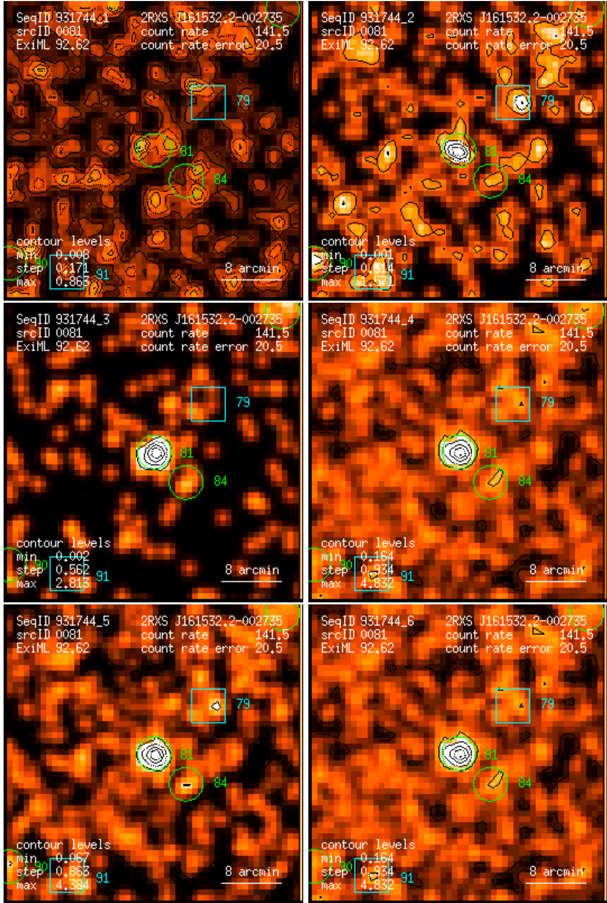
Figure 81: RASS 931744: detection 0081: band rate images, Gaussian filter: (1) PSPC channels 11 – 41, (2) 52 – 90, (3) 91 – 201, (4) 11 – 235, (5) 52 – 201, (6) 11 – 201. Broad band rates in counts/ks. Band rate contour levels in counts/ks/arcmin 2 .
