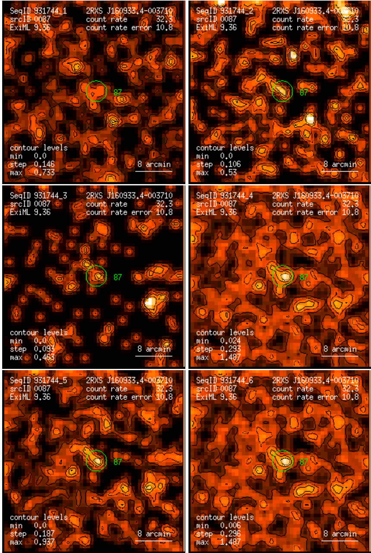
Figure 87: RASS 931744: detection 0087: band rate images, Gaussian filter: (1) PSPC channels 11 – 41, (2) 52 – 90, (3) 91 – 201, (4) 11 – 235, (5) 52 – 201, (6) 11 – 201. Broad band rates in counts/ks. Band rate contour levels in counts/ks/arcmin 2 .
