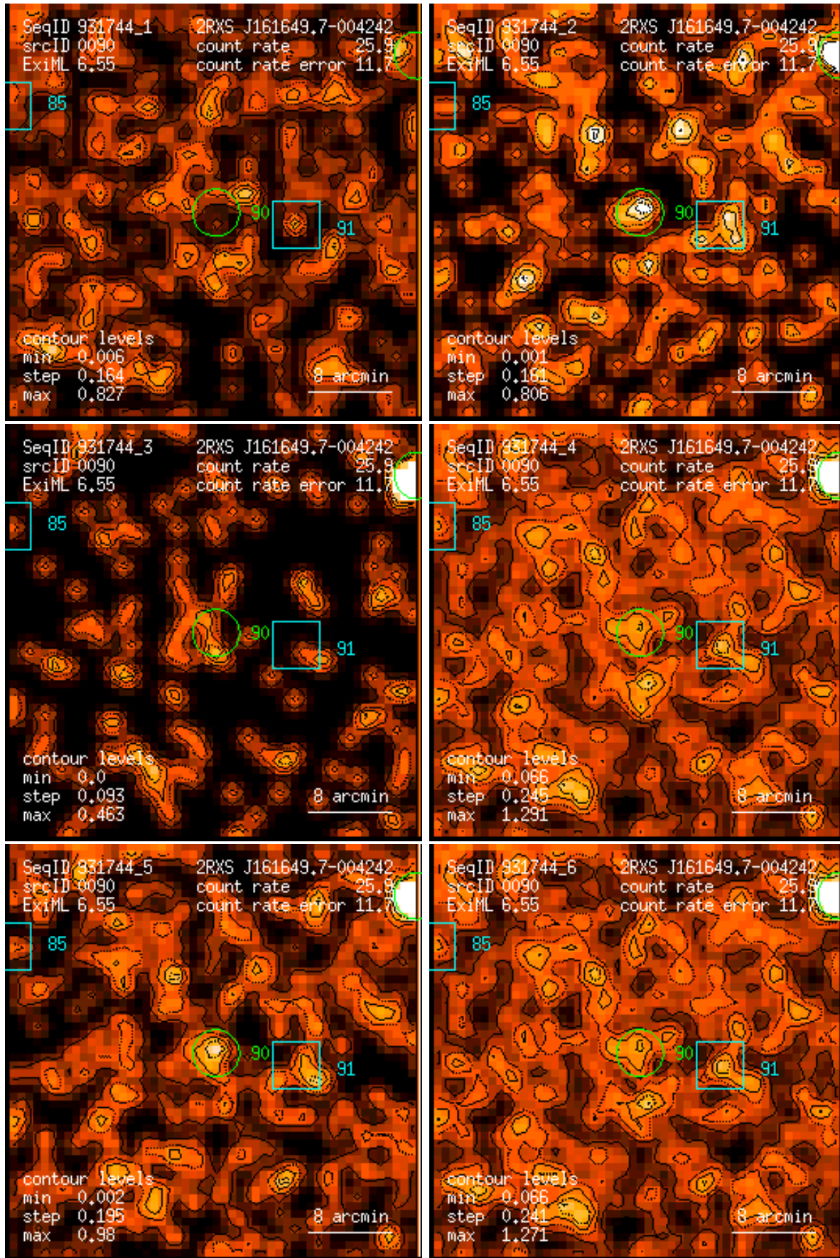
Figure 90: RASS 931744: detection 0090: band rate images, Gaussian filter: (1) PSPC channels 11 – 41, (2) 52 – 90, (3) 91 – 201, (4) 11 – 235, (5) 52 – 201, (6) 11 – 201. Broad band rates in counts/ks. Band rate contour levels in counts/ks/arcmin 2 .
