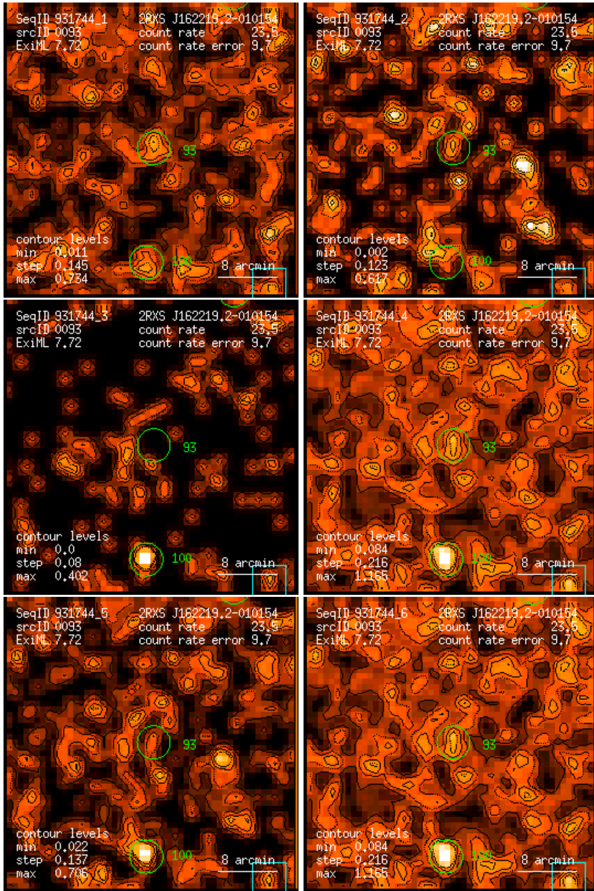
Figure 93: RASS 931744: detection 0093: band rate images, Gaussian filter: (1) PSPC channels 11 – 41, (2) 52 – 90, (3) 91 – 201, (4) 11 – 235, (5) 52 – 201, (6) 11 – 201. Broad band rates in counts/ks. Band rate contour levels in counts/ks/arcmin 2 .
