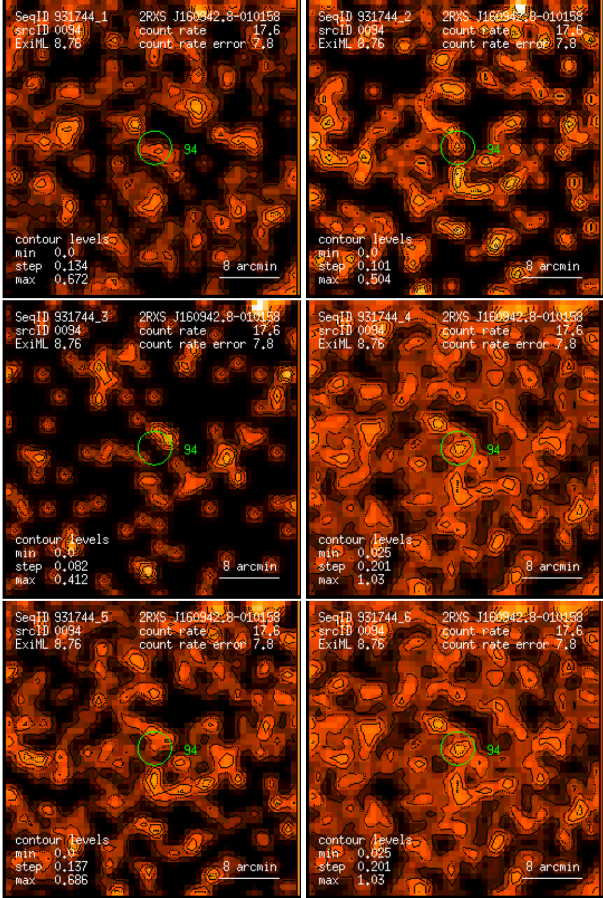
Figure 94: RASS 931744: detection 0094: band rate images, Gaussian filter: (1) PSPC channels 11 – 41, (2) 52 – 90, (3) 91 – 201, (4) 11 – 235, (5) 52 – 201, (6) 11 – 201. Broad band rates in counts/ks. Band rate contour levels in counts/ks/arcmin 2 .
