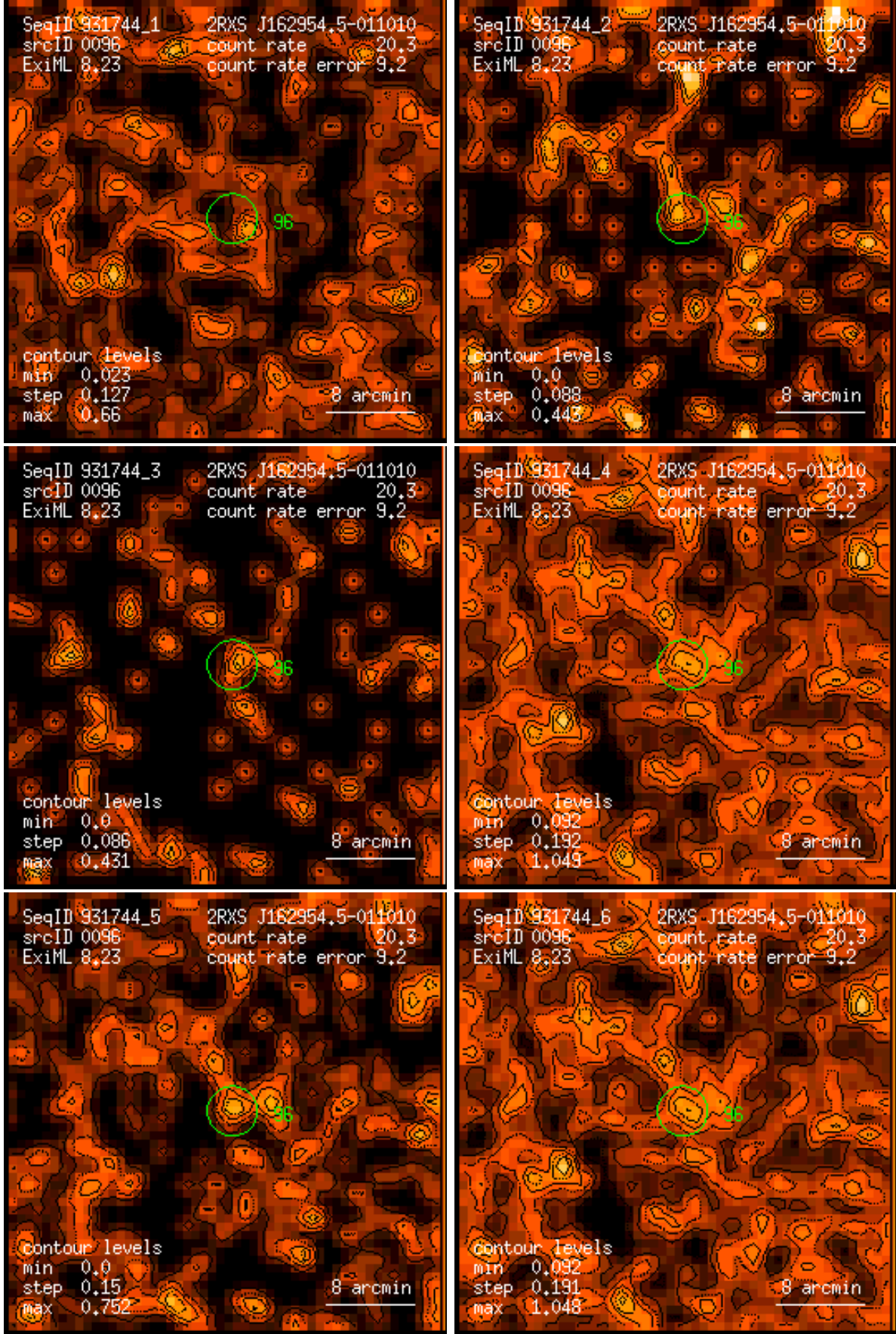
Figure 96: RASS 931744: detection 0096: band rate images, Gaussian filter: (1) PSPC channels 11 – 41, (2) 52 – 90, (3) 91 – 201, (4) 11 – 235, (5) 52 – 201, (6) 11 – 201. Broad band rates in counts/ks. Band rate contour levels in counts/ks/arcmin 2 .
