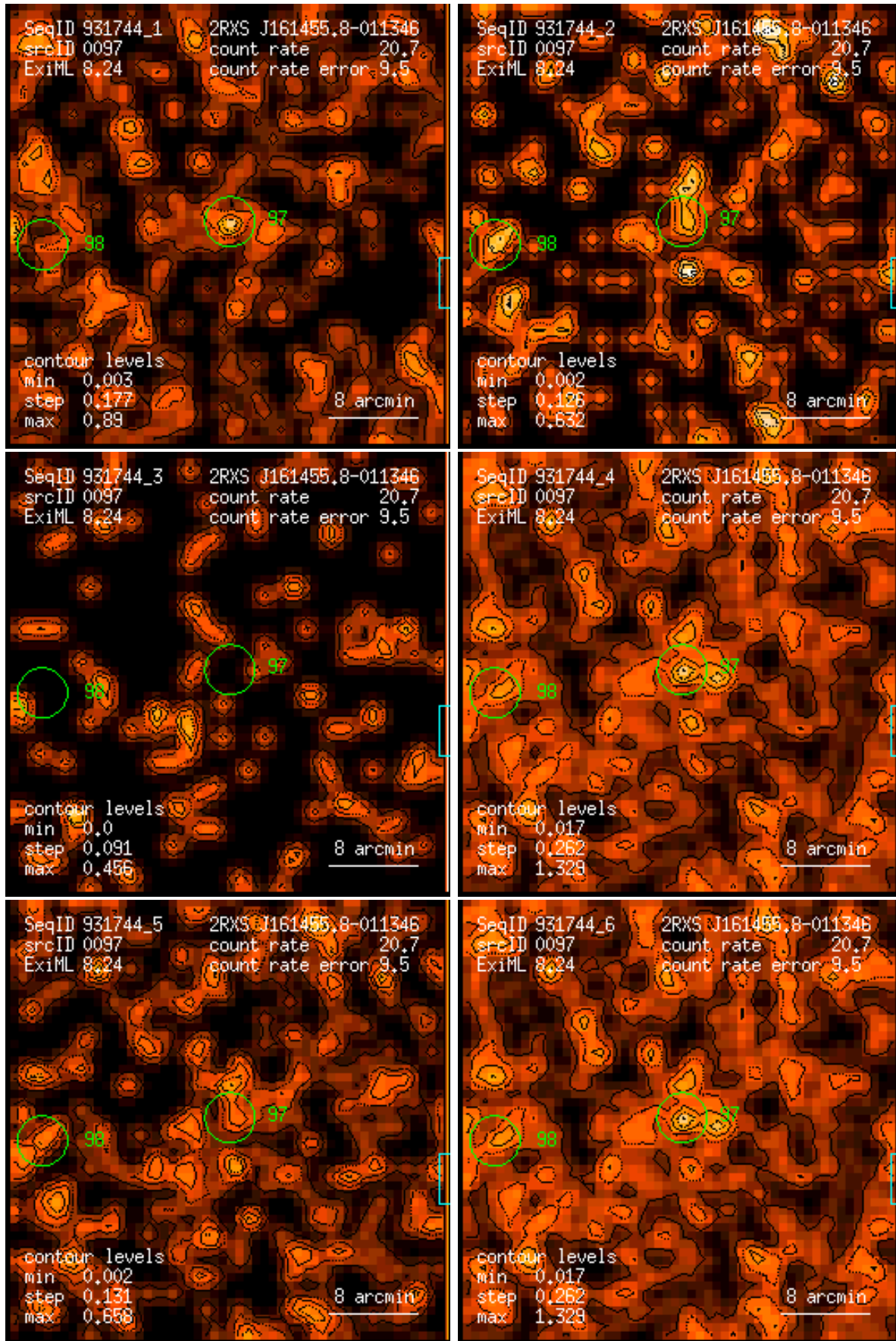
Figure 97: RASS 931744: detection 0097: band rate images, Gaussian filter: (1) PSPC channels 11 – 41, (2) 52 – 90, (3) 91 – 201, (4) 11 – 235, (5) 52 – 201, (6) 11 – 201. Broad band rates in counts/ks. Band rate contour levels in counts/ks/arcmin 2 .
