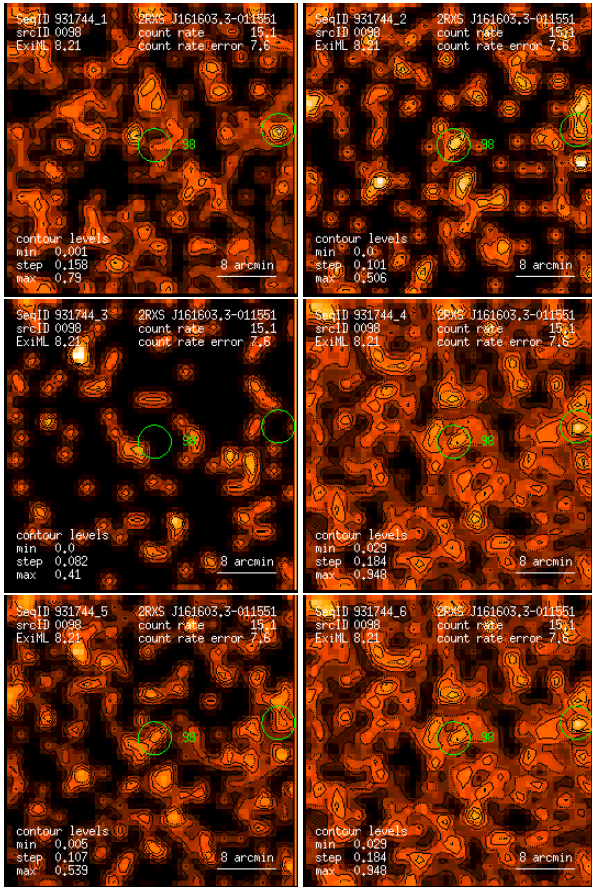
Figure 98: RASS 931744: detection 0098: band rate images, Gaussian filter: (1) PSPC channels 11 – 41, (2) 52 – 90, (3) 91 – 201, (4) 11 – 235, (5) 52 – 201, (6) 11 – 201. Broad band rates in counts/ks. Band rate contour levels in counts/ks/arcmin 2 .
