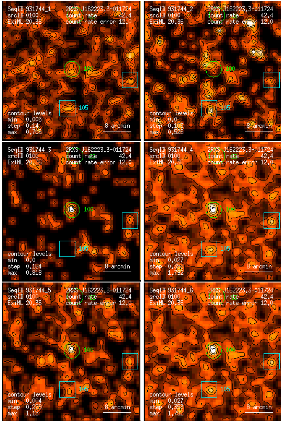
Figure 100: RASS 931744: detection 0100: band rate images, Gaussian filter: (1) PSPC channels 11 – 41, (2) 52 – 90, (3) 91 – 201, (4) 11 – 235, (5) 52 – 201, (6) 11 – 201. Broad band rates in counts/ks. Band rate contour levels in counts/ks/arcmin 2 .
