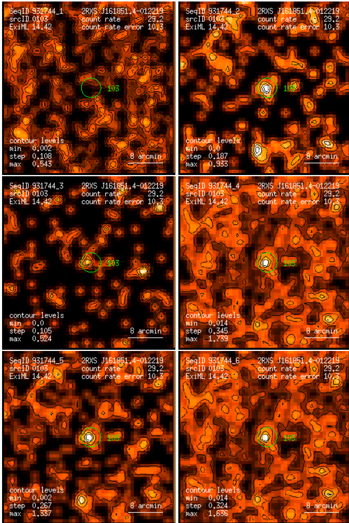
Figure 103: RASS 931744: detection 0103: band rate images, Gaussian filter: (1) PSPC channels 11 – 41, (2) 52 – 90, (3) 91 – 201, (4) 11 – 235, (5) 52 – 201, (6) 11 – 201. Broad band rates in counts/ks. Band rate contour levels in counts/ks/arcmin 2 .
