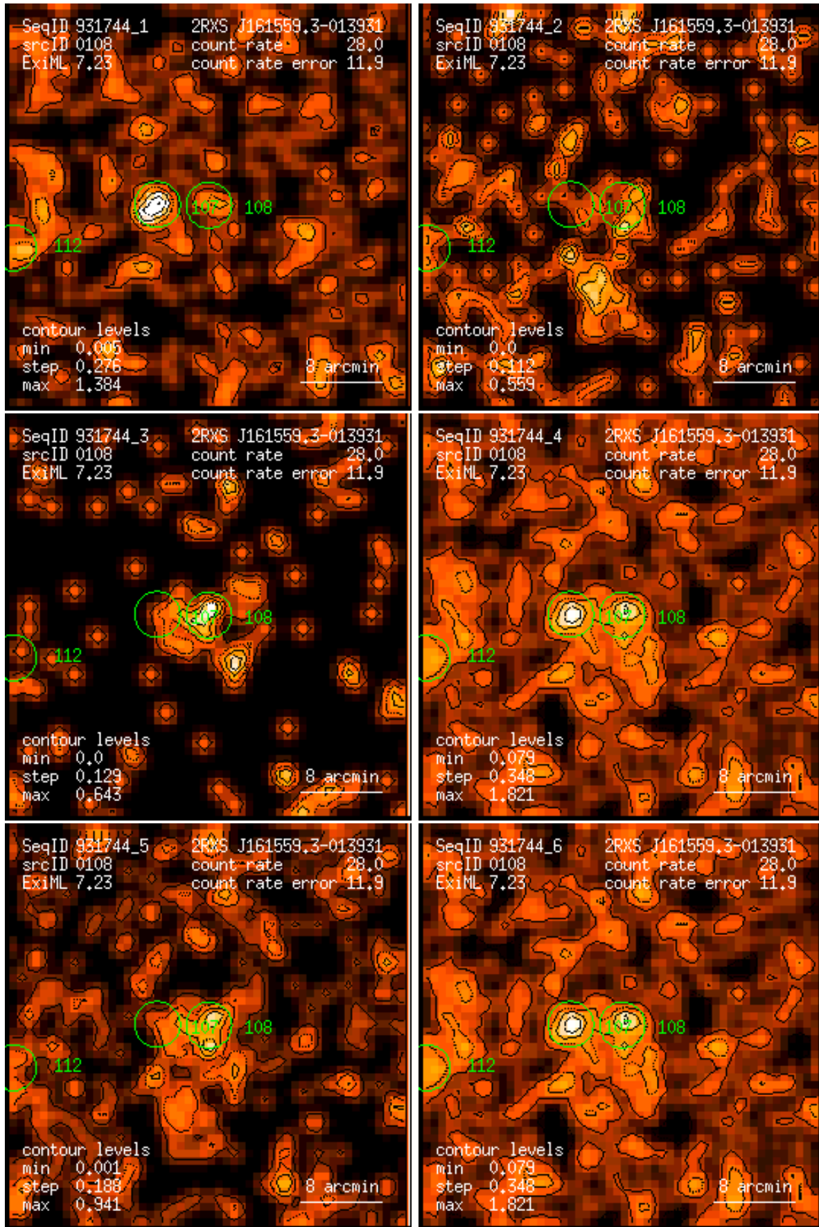
Figure 108: RASS 931744: detection 0108: band rate images, Gaussian filter: (1) PSPC channels 11 – 41, (2) 52 – 90, (3) 91 – 201, (4) 11 – 235, (5) 52 – 201, (6) 11 – 201. Broad band rates in counts/ks. Band rate contour levels in counts/ks/arcmin 2 .
