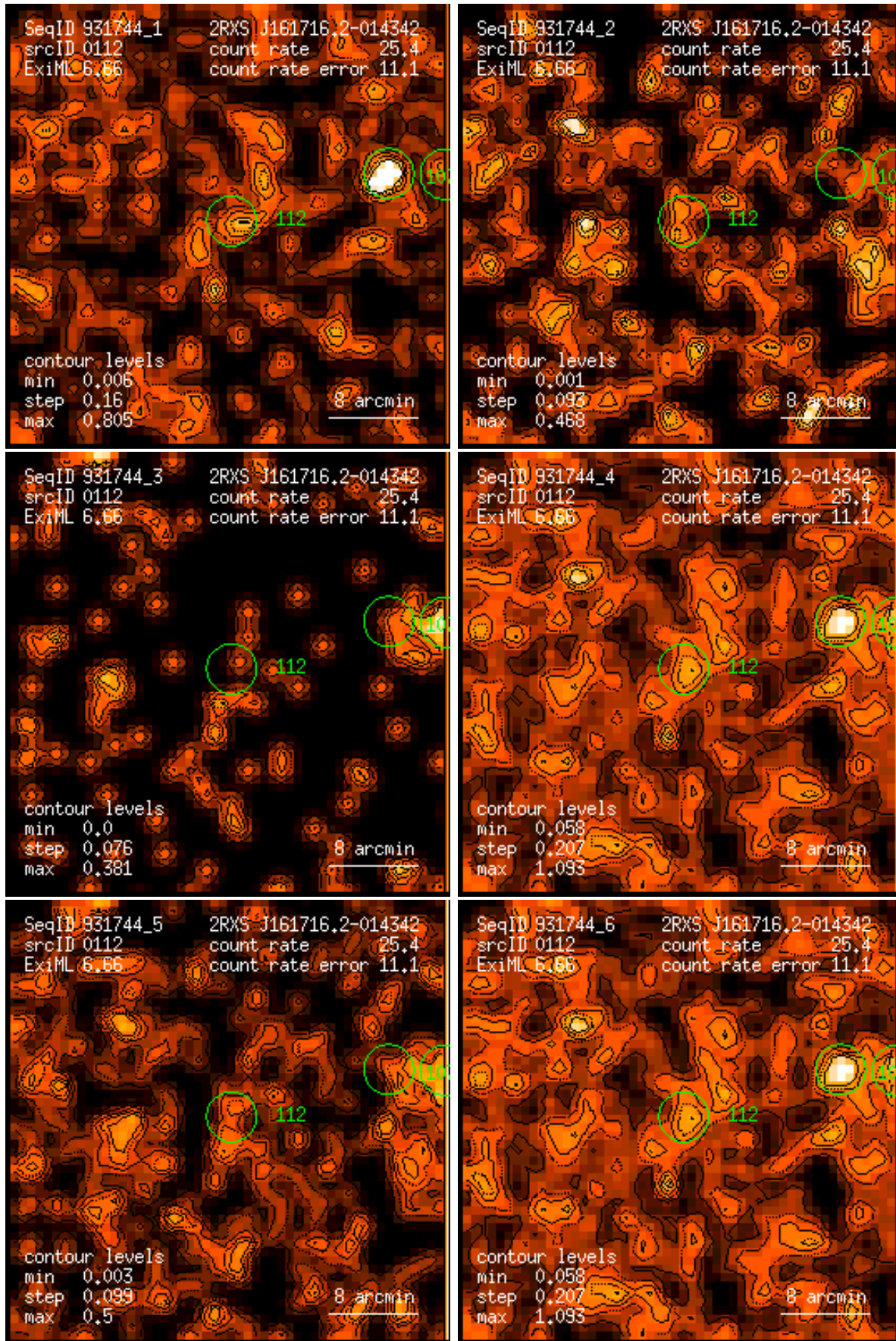
Figure 112: RASS 931744: detection 0112: band rate images, Gaussian filter: (1) PSPC channels 11 – 41, (2) 52 – 90, (3) 91 – 201, (4) 11 – 235, (5) 52 – 201, (6) 11 – 201. Broad band rates in counts/ks. Band rate contour levels in counts/ks/arcmin 2 .
