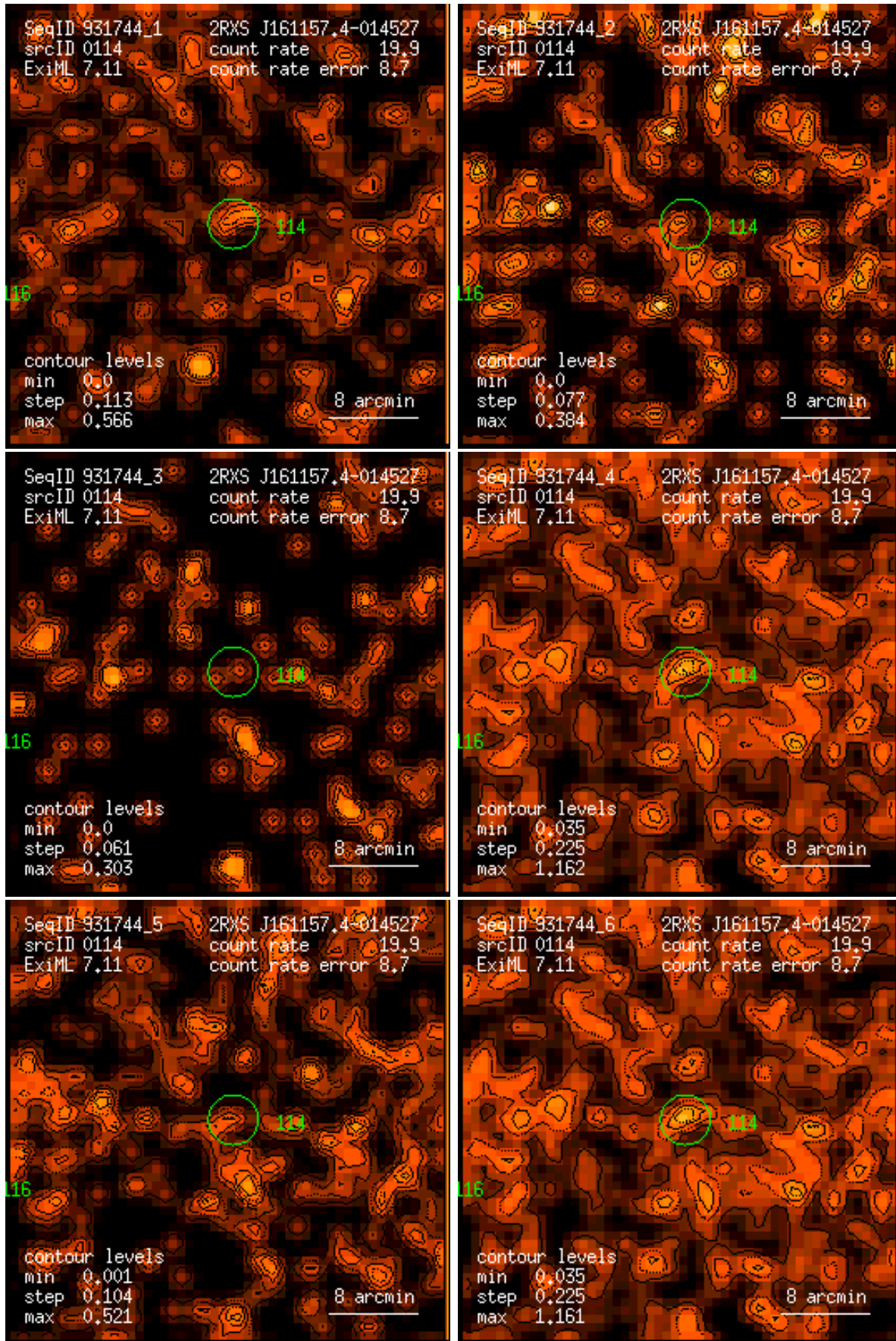
Figure 114: RASS 931744: detection 0114: band rate images, Gaussian filter: (1) PSPC channels 11 – 41, (2) 52 – 90, (3) 91 – 201, (4) 11 – 235, (5) 52 – 201, (6) 11 – 201. Broad band rates in counts/ks. Band rate contour levels in counts/ks/arcmin 2 .
