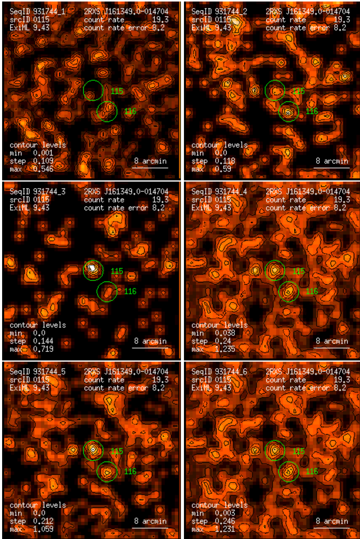
Figure 115: RASS 931744: detection 0115: band rate images, Gaussian filter: (1) PSPC channels 11 – 41, (2) 52 – 90, (3) 91 – 201, (4) 11 – 235, (5) 52 – 201, (6) 11 – 201. Broad band rates in counts/ks. Band rate contour levels in counts/ks/arcmin 2 .
